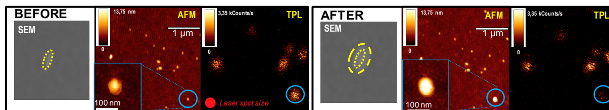
Figure 3. Correlated topography and TPL images of a sample of GNR immobilized onto an ITO coated glass cover slide, BEFORE and AFTER the “over-illumination” ( F = 125 \mu\text{J}\cdot\text{cm}^{-2} , \lambda = 800 nm) of the blue circled GNR. High resolution tapping mode AFM scans of the blue circled GNR are displayed as insets of the topography scans, together with complementary SEM images.
