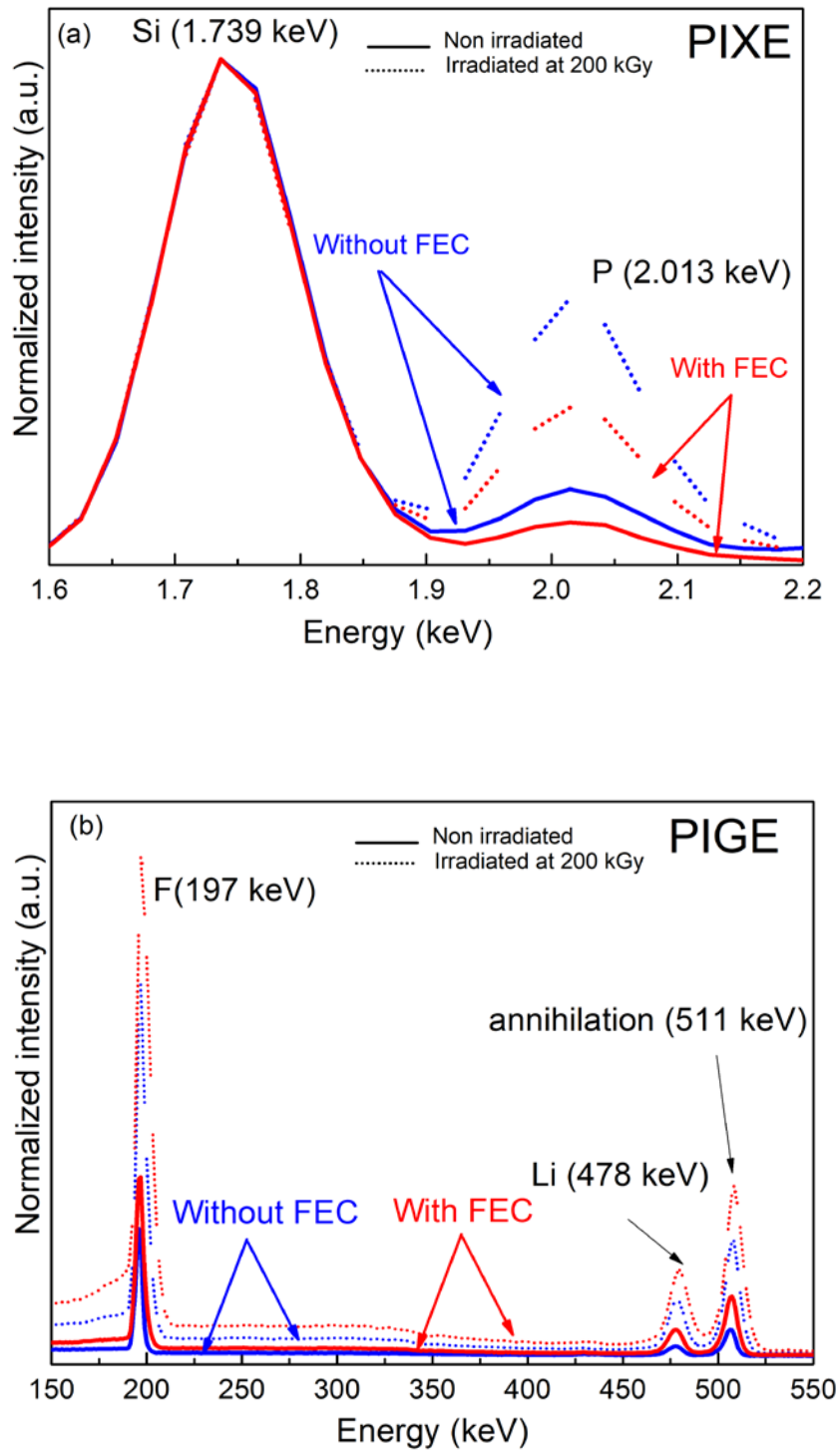
Figure 1. Evolution of the PIXE (a) and PIGE (b) spectra of the Si NPs/electrolyte system before (line) and after irradiation at 200 kGy (dotted line). Blue and red colors are used for the samples exposed/irradiated to/in electrolytes without or with FEC, respectively. For the sake of comparison, each spectrum is normalized with respect to the Si signal.
