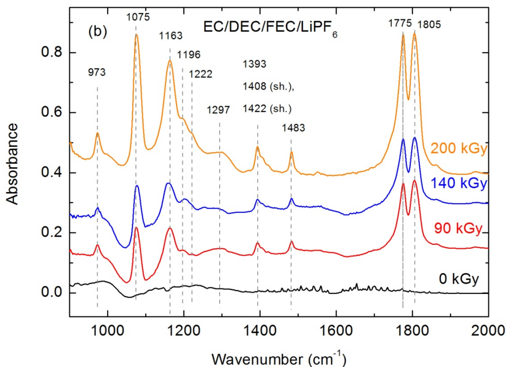
Figure 3. Evolution of IR spectra in the 900-2000 \text{cm}^{-1} wavenumber range before and after irradiation at increasing doses for the Si NPs/electrolyte system: (a) EC/DEC/LiPF 6 ; (b) EC/DEC/FEC/LiPF 6 . “sh.” stands for shoulder. The characteristic wavenumbers are displayed on the figures. As stated in the experimental section, no quantitative information can be obtained from these spectra. The spectra were thus rescaled for the sake of clarity.
