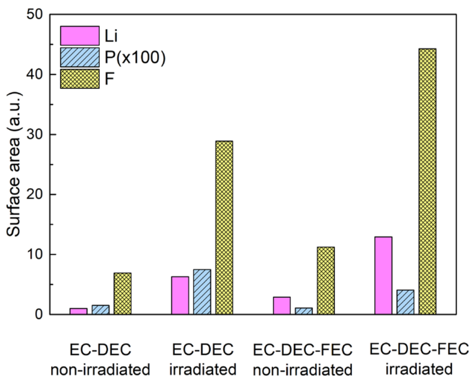
Figure 2. Evolution of the surface area corresponding to the elemental peak (PIXE P 2.013 keV; PIGE F: 197 keV and Li: 478 keV) for the Si NPs/electrolyte systems (with and without FEC) before and after irradiation at 200 kGy.
