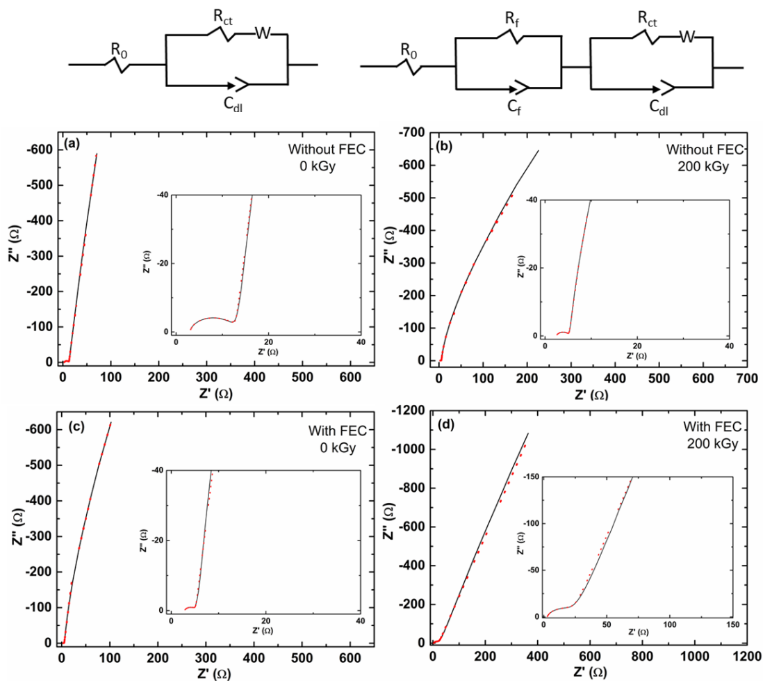
Figure 7. Electrochemical impedance spectroscopy (EIS) raw spectra of the symmetrical cells containing silicon nanoparticles before (a, c) and after (b, d) irradiation at a dose of 200 kGy ((a and b) without FEC and (c and d) with FEC). The inset in the figures (a to d) is a focus on the lowest Z' values. The corresponding electrical equivalent circuits before (left) and after (right) irradiation are shown above. The electrical equivalent circuit contains less parameters before than after irradiation, as no SEI is observed when the samples are not irradiated.
