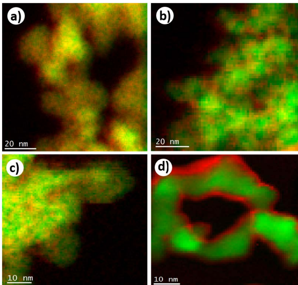
Figure 6. STEM images and EELS mapping of Si nanoparticles after (a) exposure to EC/DEC/LiPF 6 electrolyte; (b) irradiation at 190 kGy in a EC/DEC/LiPF 6 electrolyte; (c) exposure to EC/DEC/FEC/LiPF 6 electrolyte; (d) irradiation at 200 kGy in a EC/DEC/FEC/LiPF 6 electrolyte. The green color stands for silicon and the red one for carbon. The yellow color arises from regions with less carbon amount than the red ones.
