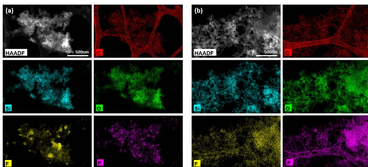
Figure 4. EDX images of the silicon nanoparticles (a) non-irradiated but exposed to EC/DEC/LiPF 6 ; (b) irradiated at 200 kGy in EC/DEC/LiPF 6 . Carbon is in red; silicon in pale blue; oxygen in green; fluorine in yellow and phosphorus in purple.
