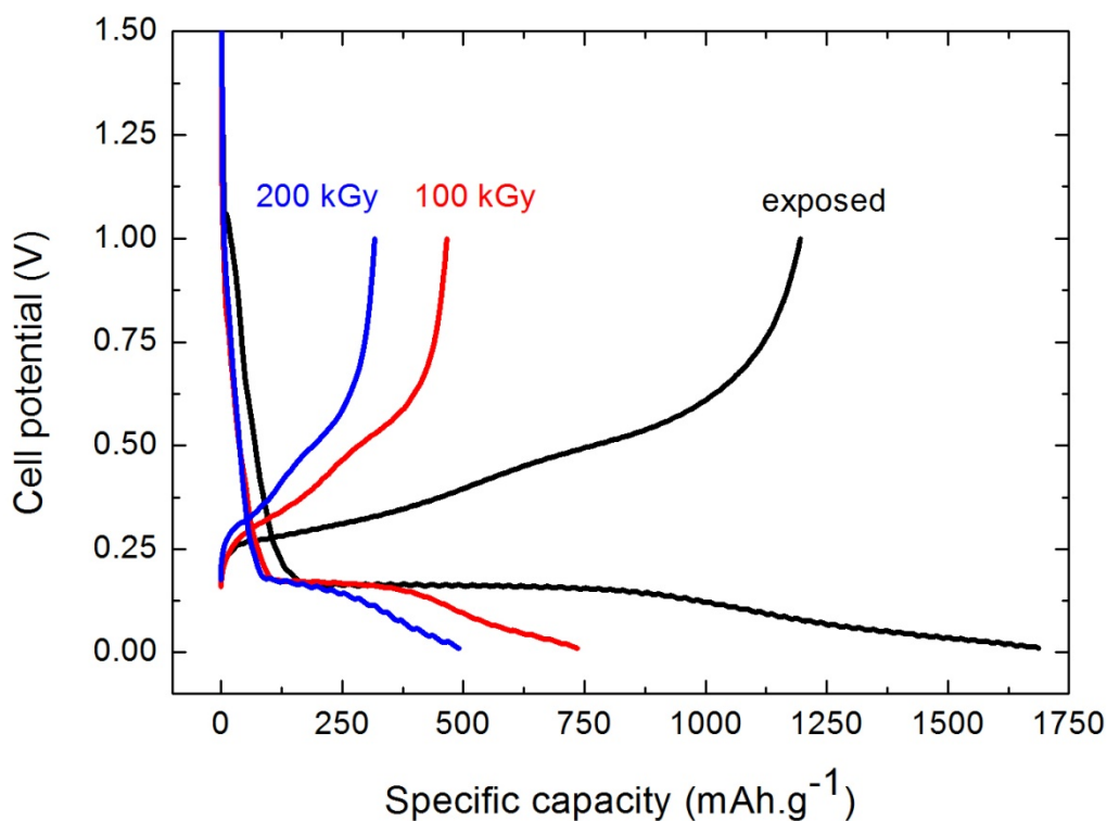
Figure 8. First cycle potential vs. specific capacity curve for the Si NPs exposed to the electrolyte containing FEC (black) and not irradiated; and after irradiation in the same electrolyte at a total dose of 100 kGy (red) and 200 kGy (blue).
