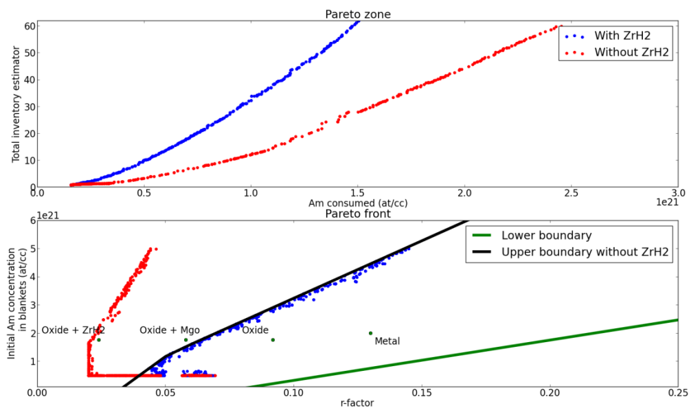
Figure 12 : Pareto zone and front for a washing limit corresponding to 7.5 kW per assembly. The upper boundary line corresponds the achievable (Am,r) range not considering the use of zirconium hydride. Green dots are corresponding to cores described in Table 9.
