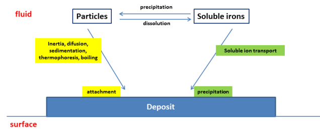
Figure 5: Phenomena governing SG deposits
