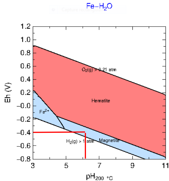
Figure 4: Pourbaix diagram for iron at 200 °C calculated with PHREEQCEA; \text{pH}_{25\text{ }^\circ\text{C}} > 9 corresponds to \text{pH}_{200\text{ }^\circ\text{C}} > 6 .
