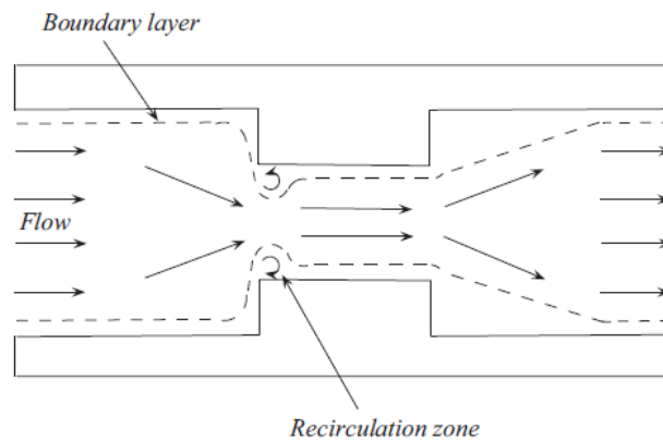
Figure 6: Pattern of vena contracta region [1,69]
