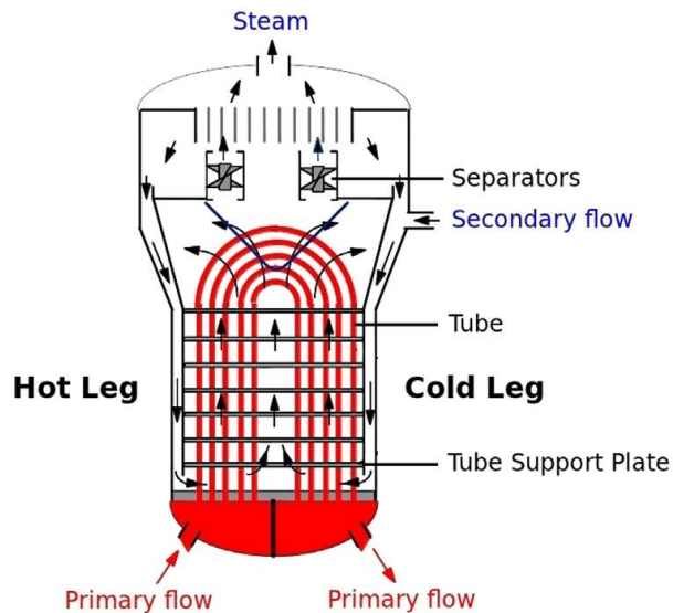
Figure 1: PWR recirculating steam generator [1]
