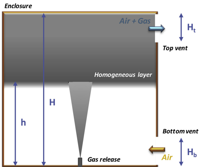
Fig. 1 – Scheme of the dispersion phenomenon considered in a naturally ventilated enclosure with two openings located at different altitudes.
