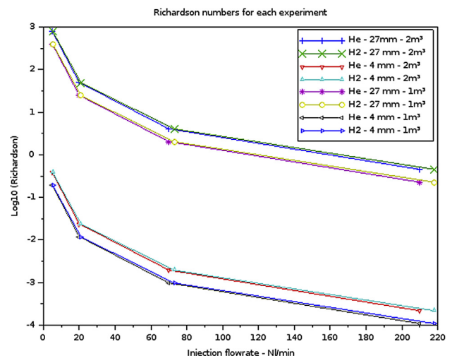
Fig. 5 – Richardson numbers.
