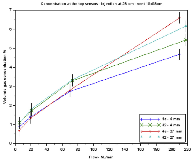
Fig. 7 – Helium and hydrogen release – Maximum volume concentrations at different flow rates and for 4 mm and 27 mm injection diameters.
