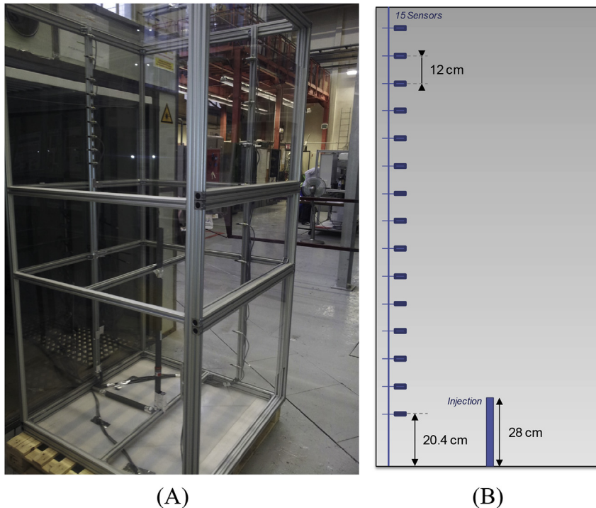
Fig. 2 – Grand-Gamelan 2-m 3 build-up enclosure. (A) Picture of the enclosure, (B) location of the sensors in the enclosure.
