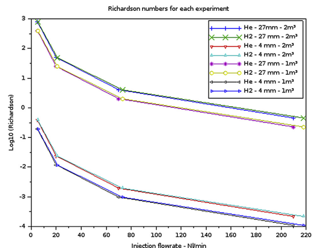
Fig. 5 – Richardson numbers.
