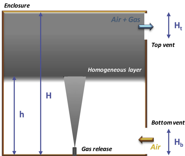
Fig. 1 – Scheme of the dispersion phenomenon considered in a naturally ventilated enclosure with two openings located at different altitudes.
