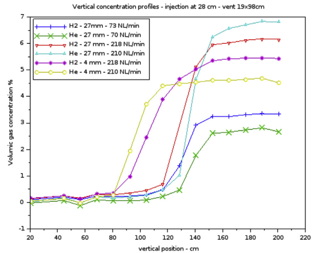
Fig. 8 – Vertical concentration profiles at different flow rates and injection diameter for helium and hydrogen.
