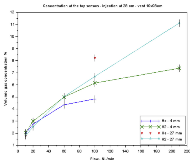
Fig. 9 – Maximum concentrations for helium and hydrogen injection in the 1-m 3 enclosure.
