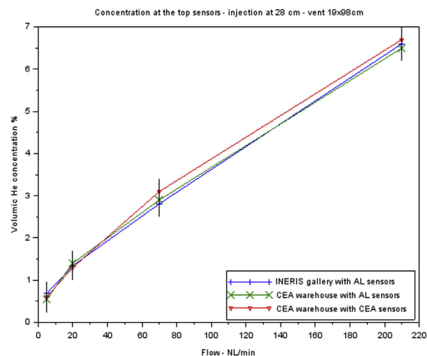
Fig. 6 – Maximum concentration of helium at the top of the enclosure for different flow rates and for 3 tests campaigns. Exp. I is located at INERIS, Exp. II at CEA and Exp. III at CEA but with CEA's own sensors.
