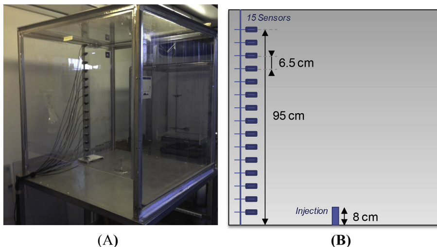
Fig. 3 – 1-m 3 build-up enclosure. (A) Picture of the enclosure, (B) location of the sensors in the enclosure.
