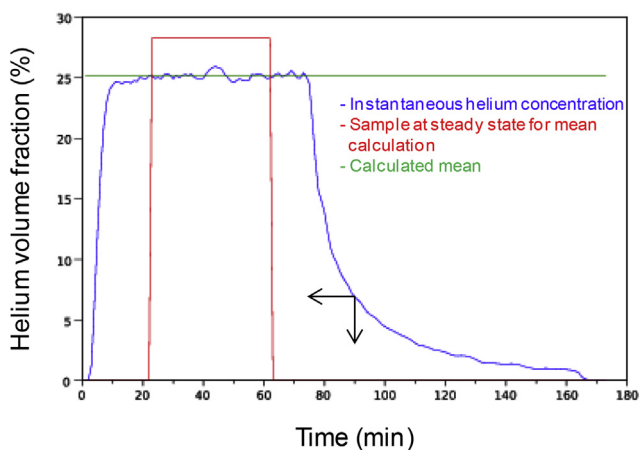
Fig. 4 – Data treatment for steady state determination based on time-measured helium volume fraction.
