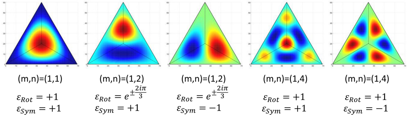
Fig. 3. Some eigenfunctions of the Laplacian operator in the equilateral triangle.
