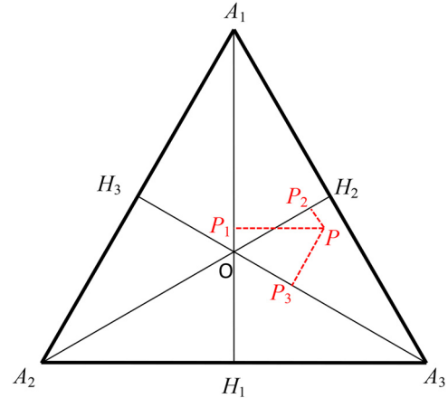
Fig. A.1. Lamé’s coordinates of point P in the equilateral triangle are such that u = A_1P_1 - 2r, v = A_2P_2 - 2r , and w = A_3P_3 - 2r ( r being the inradius of the triangle and P_1, P_2 , and P_3 being, respectively, the orthogonal projections of P onto A_1H_1, A_2H_2 , and A_3H_3 ). Examples are O(0, 0, 0) , A_1(-2r, 0, 0) , and H_1(r, -r/2, -r/2) .
