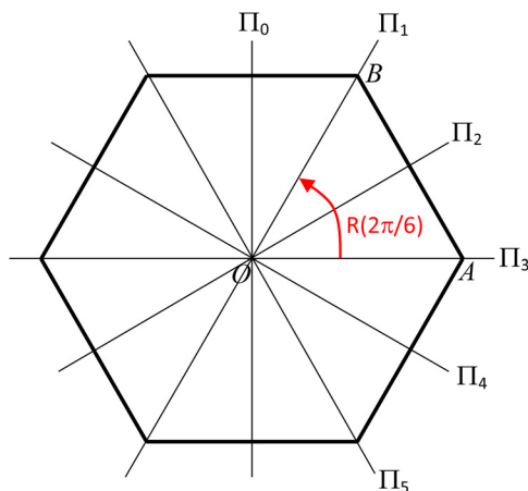
Fig. 2. Cross section of a prismatic hexagonal homogeneous system with a trace of the mirror symmetry planes ( \Pi_0 to \Pi_5 ), with \pi/6 clockwise angle between one and the next. R = S_0 S_1 is the counterclockwise rotation of angle 2\pi/6 .
