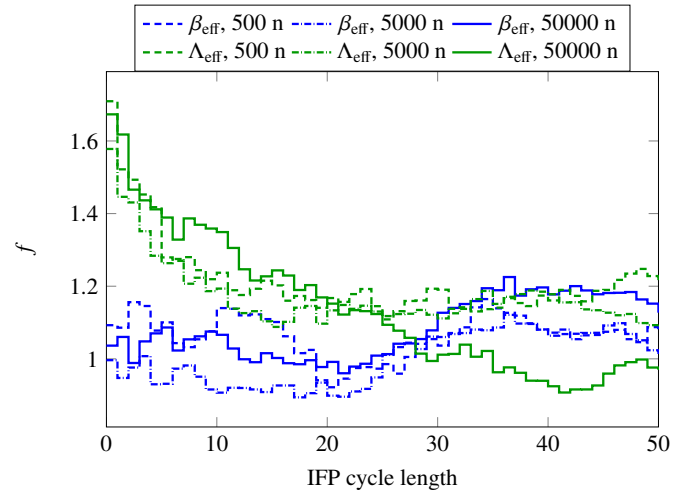
Figure 8: Inter-cycle correlations on \beta_{\text{eff}} and \Lambda_{\text{eff}} for the N4 PWR reactor. The factor f = \hat{\sigma}/\hat{\sigma}_a is plotted as a function of the IFP cycle length M . Large deviations from f \approx 1 imply strong inter-cycle correlations.
