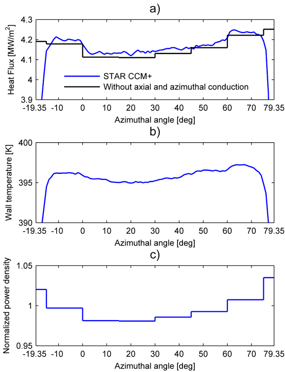
Figure 15: Hot channel calculation azimuthal dependent heat flux (a) and wall temperature (b) on the first fuel plate and the normalized power density (c) in the fuel meat at the height z = 0.315 m. All the parameters are plotted in the azimuthal interval that corresponds to the fuel meat location.
