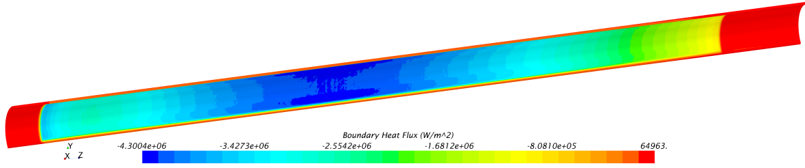
Figure 14: Boundary heat flux on the hot channel. Flow direction is from the left to the right and boundaries are seen from the center of the fuel assembly.
