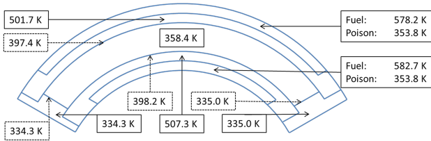
Figure 12: Schematic view of the maximum temperatures in the hot channel calculation. Dashed box marks the water-solid interface. Arrow shows only the part not the specific location.
