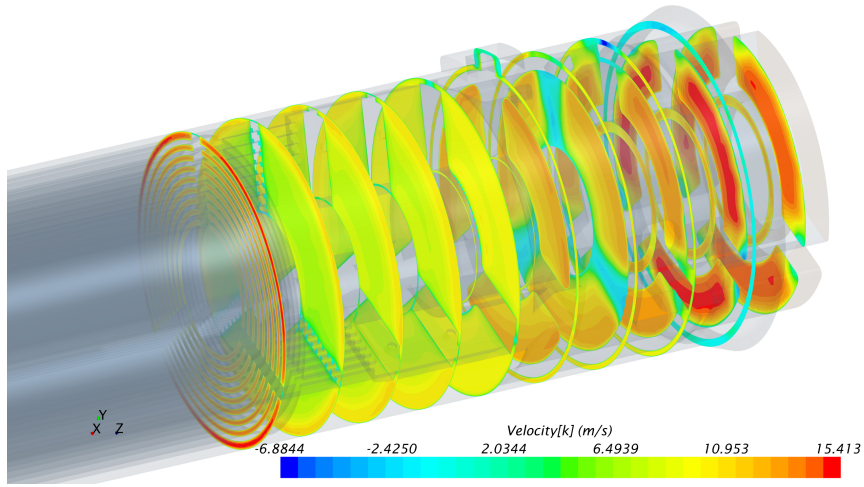
Figure 8: Top end cap surrounding flow field velocity axial components illustrated on multiple plane sections separated by 2.0 cm.
