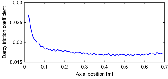
Figure 10: Darcy friction coefficient in the hot channel of the full fuel assembly geometry.
