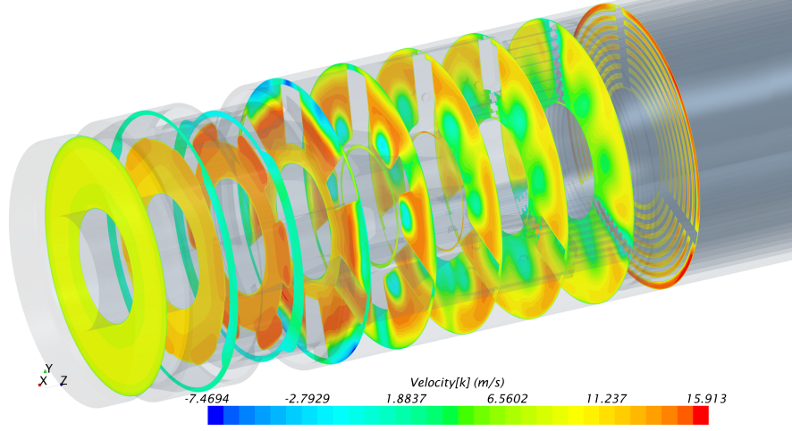
Figure 6: Bottom end cap surrounding flow field velocity axial components illustrated on multiple plane sections separated by 2.5 cm.
