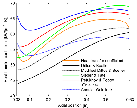
Figure 17: Heat transfer coefficient obtained in the hot channel compared with the correlations.
