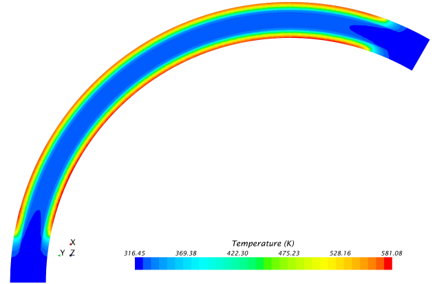
Figure 16: Temperature distribution in the hot channel and in the surrounding metal structures on the z = 0.315 m plane.
