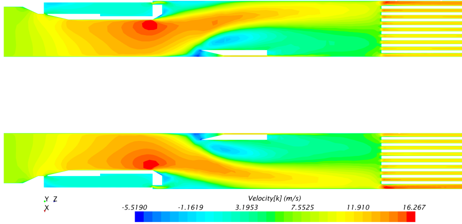
Figure 7: Velocity axial components around bottom end cap on the plate y=0 .
