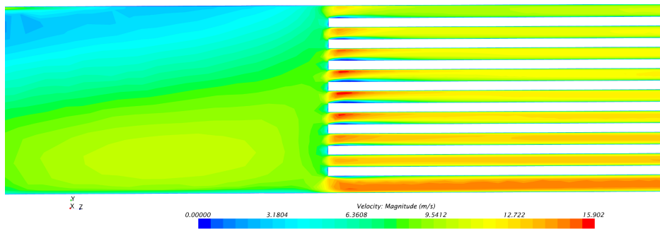
Figure 11: Velocity around bottom end cap in the center of hot sector on the plate x=0 .
