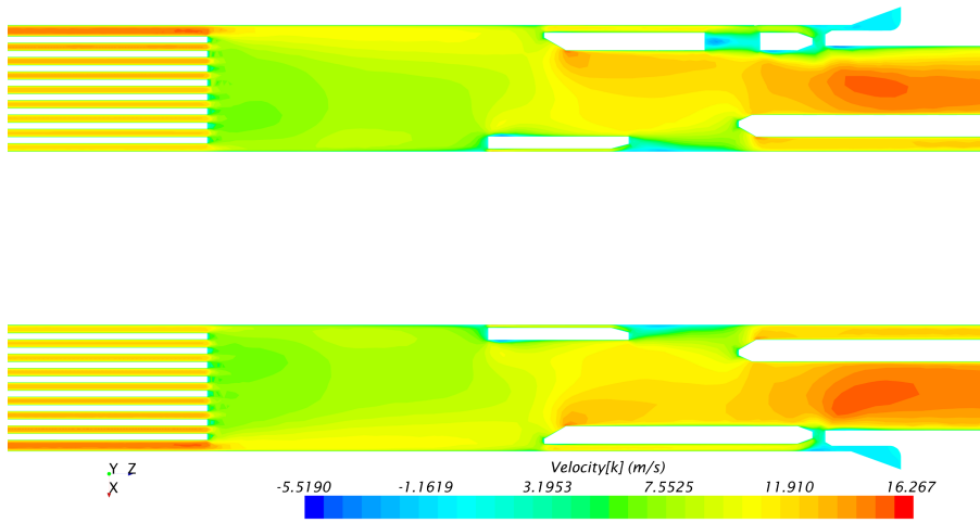
Figure 9: Velocity axial components around top end cap on the plate y=0 .
