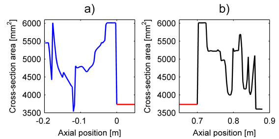
Figure 3: Cross-section areas of the flow surrounding the bottom end cap (a) and the top end cap (b). Red color marks flow cross-section area through the fuel plates.
