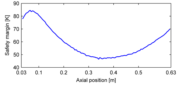
Figure 13: Safety margin in the hot channel in a fuel meat zone.
