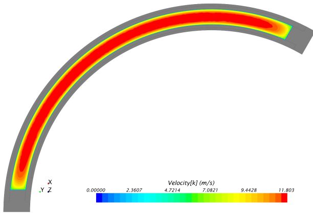
Figure 5: Velocity distribution in the hot channel on the z = 0.315 m plane.
