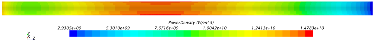
Figure 4: Power density distribution in the first fuel plate meat in the hot channel calculation. Flow direction is from the left to the right and fuel meat is seen from the center of the fuel assembly.
