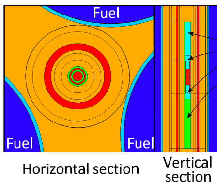
Figure 7: Horizontal and vertical sections of the computational models used in the calculations. Left: MIC inserted into MP25 in the computational model of the JSI TRIGA Mark II reactor, first phase of calculations. Right: computational model of a MIC, second phase of calculations.
