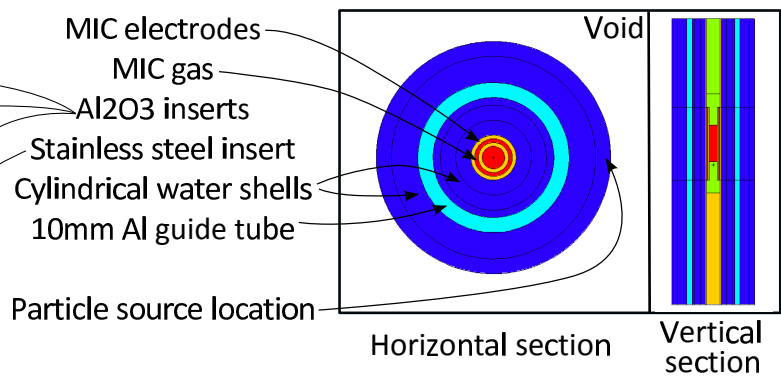
Figure 7: Horizontal and vertical sections of the computational models used in the calculations. Left: MIC inserted into MP25 in the computational model of the JSI TRIGA Mark II reactor, first phase of calculations. Right: computational model of a MIC, second phase of calculations.
