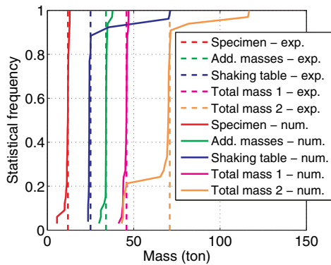
(a) Empirical distribution of some mass based indicators
