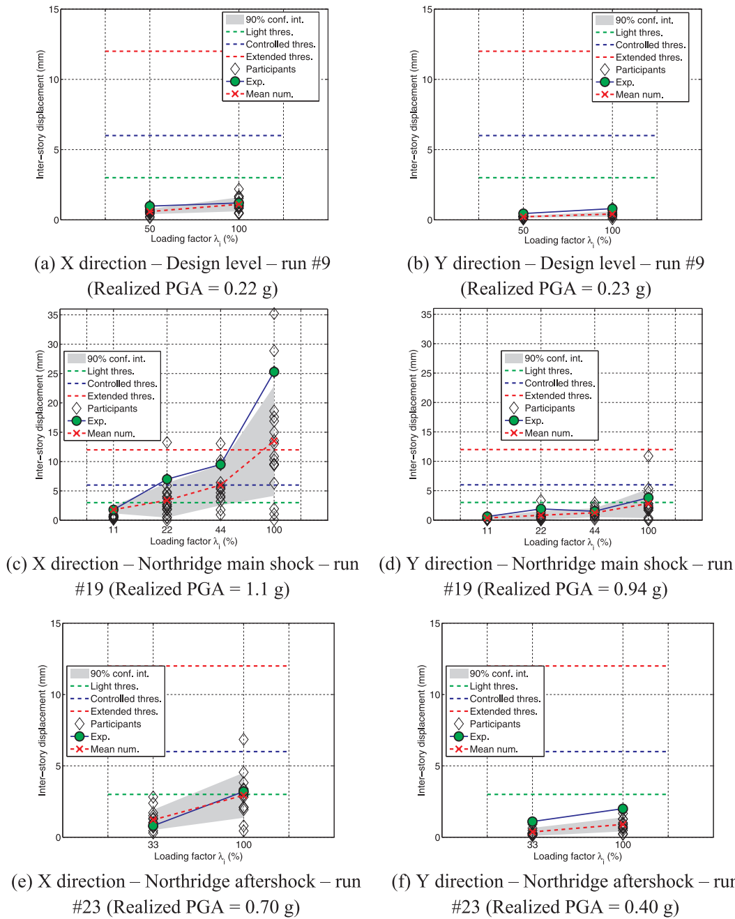
Fig. 11. Seismic safety margins based on a displacement based indicator – experimental/numerical comparisons, computed on the participants' pool.
