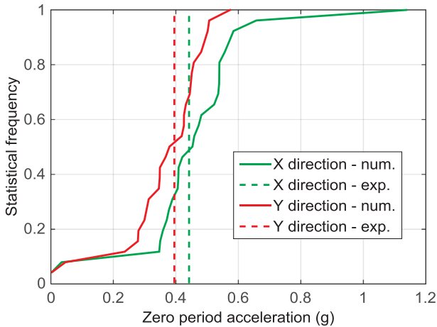
Fig. 9. Empirical cumulative distribution function of the ZPA – third floor – point D – run #7, computed on the participants' pool.
