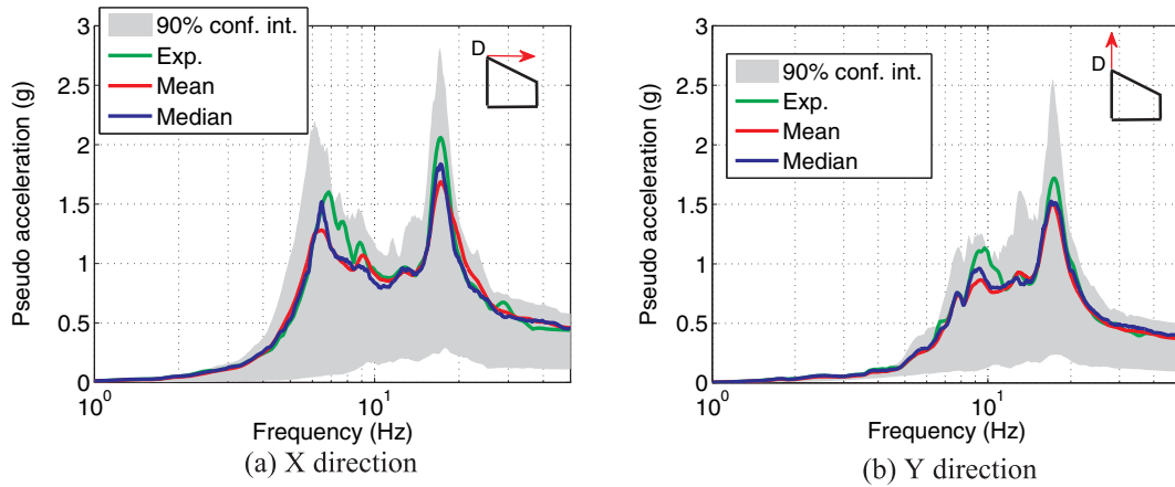
Fig. 8. Experimental/numerical comparison of the FRS – third floor – point D – run #7.
