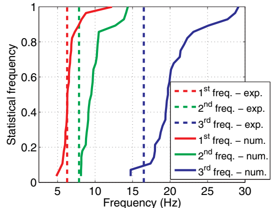
Fig. 7. Empirical cumulative distribution functions of the first three eigenfrequencies.
