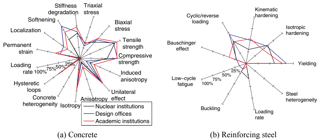
Fig. 5. Key mechanisms used by participants in connection with their origin to describe the material behaviors – percentage with respect to the total number of participants.
