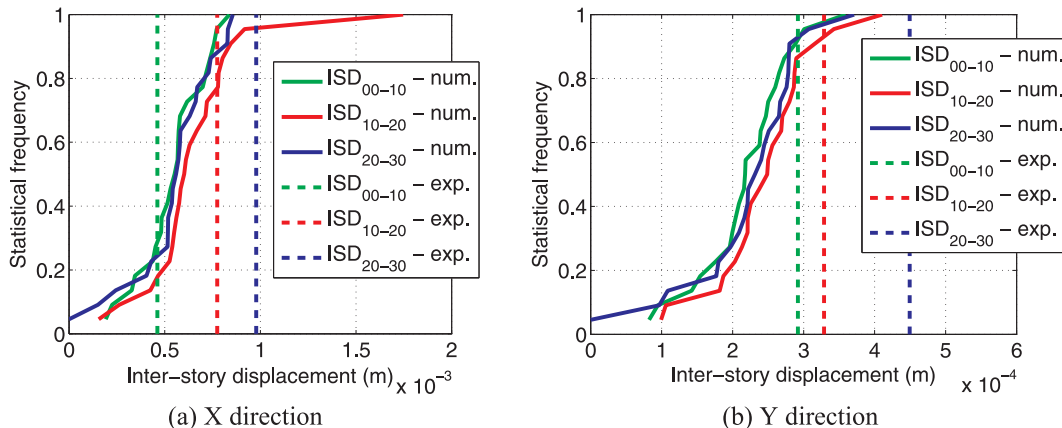
Fig. 10. Empirical cumulative distribution functions of the maximum absolute values of the ISD – point D – run #7, computed on the participants' pool.
