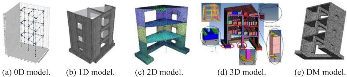
Fig. 2. Examples of FE meshes used by the participants.
