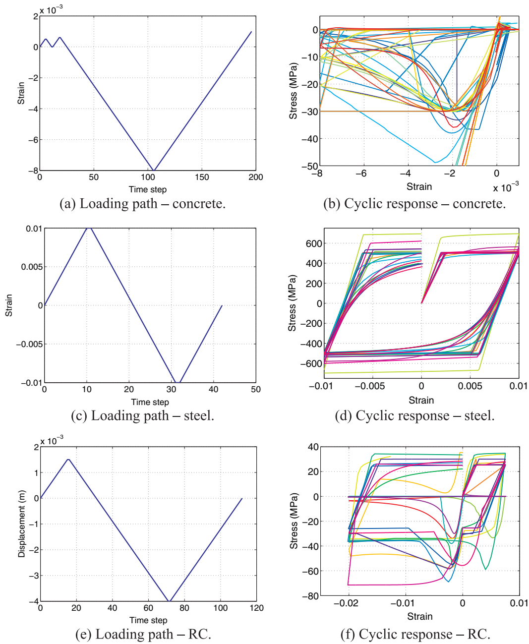
Fig. 6. Local cyclic uniaxial responses of RVEs by participants.
