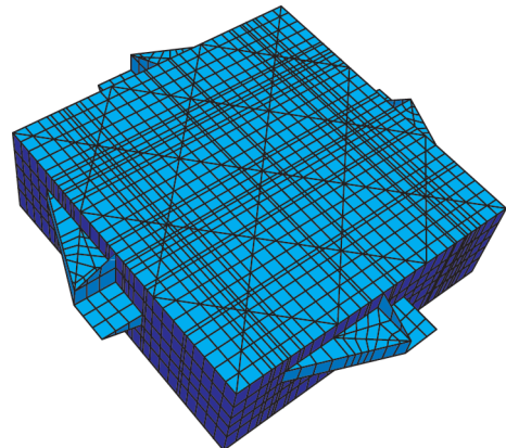
Fig. 3. Mesh of the shaking table model provided by CEA.
