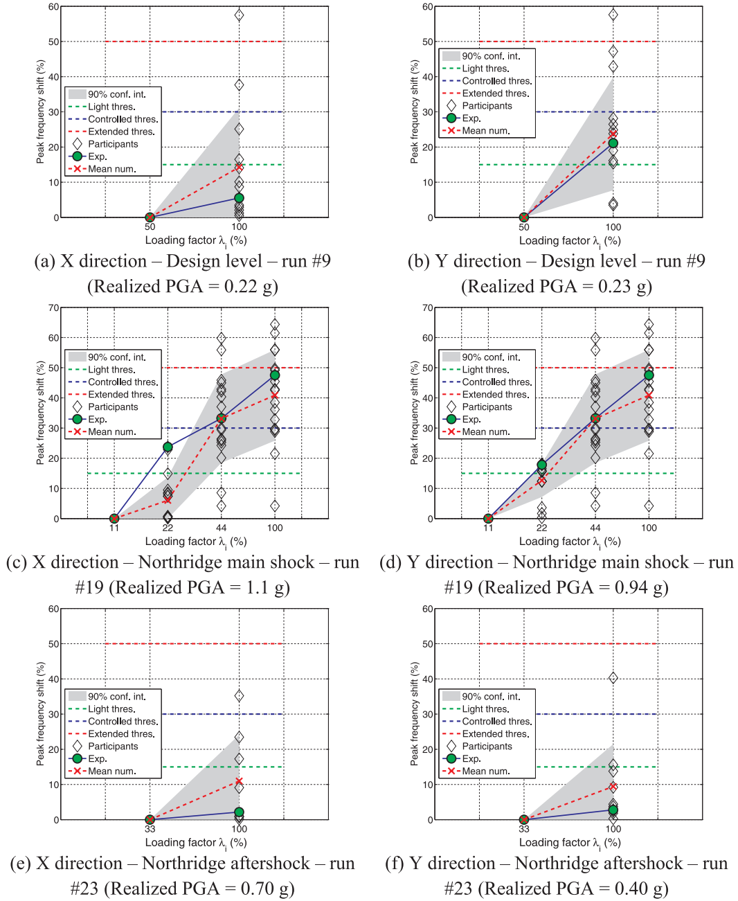
Fig. 12. Seismic safety margins based on a peak frequency based indicator – experimental/numerical comparisons, computed on the participants’ pool.
