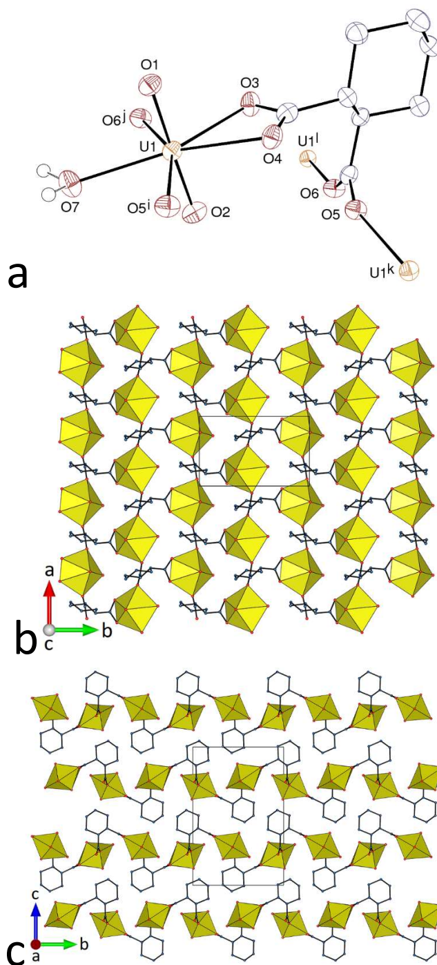
Figure 3. (a) View of compound 3 . Displacement ellipsoids are drawn at the 50% probability level. Carbon-bound hydrogen atoms are omitted. Symmetry codes: i = 1 - x, y - 1/2, 3/2 - z ; j = -x, y - 1/2, 3/2 - z ; k = 1 - x, y + 1/2, 3/2 - z ; l = -x, y + 1/2, 3/2 - z . (b) View of the 2D honeycomb-type assembly. (c) Packing with layers viewed edge-on.
