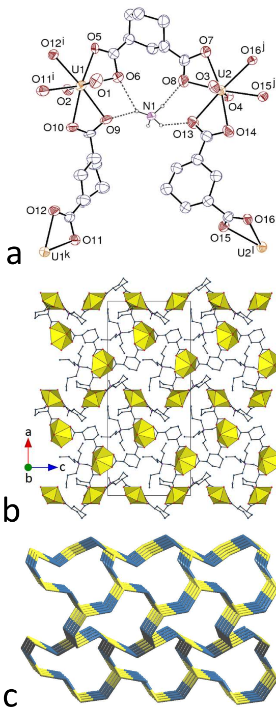
Figure 5. (a) View of compound 5. Displacement ellipsoids are drawn at the 20% probability level. Carbon-bound hydrogen atoms and \text{NBu}_4^+ cations are omitted, and hydrogen bonds are shown as dashed lines. Symmetry codes: i = 3/2 - x, y + 1/2, z - 1/2 ; j = 1 - x, -y - 1, z - 1/2 ; k = 3/2 - x, y - 1/2, z + 1/2 ; l = 1 - x, -y - 1, z + 1/2 . (b) View of the 3D framework. (c) Nodal representation of the framework (uranium, yellow; dicarboxylate ligand, dark blue; orientation slightly rotated with respect to that in b).
