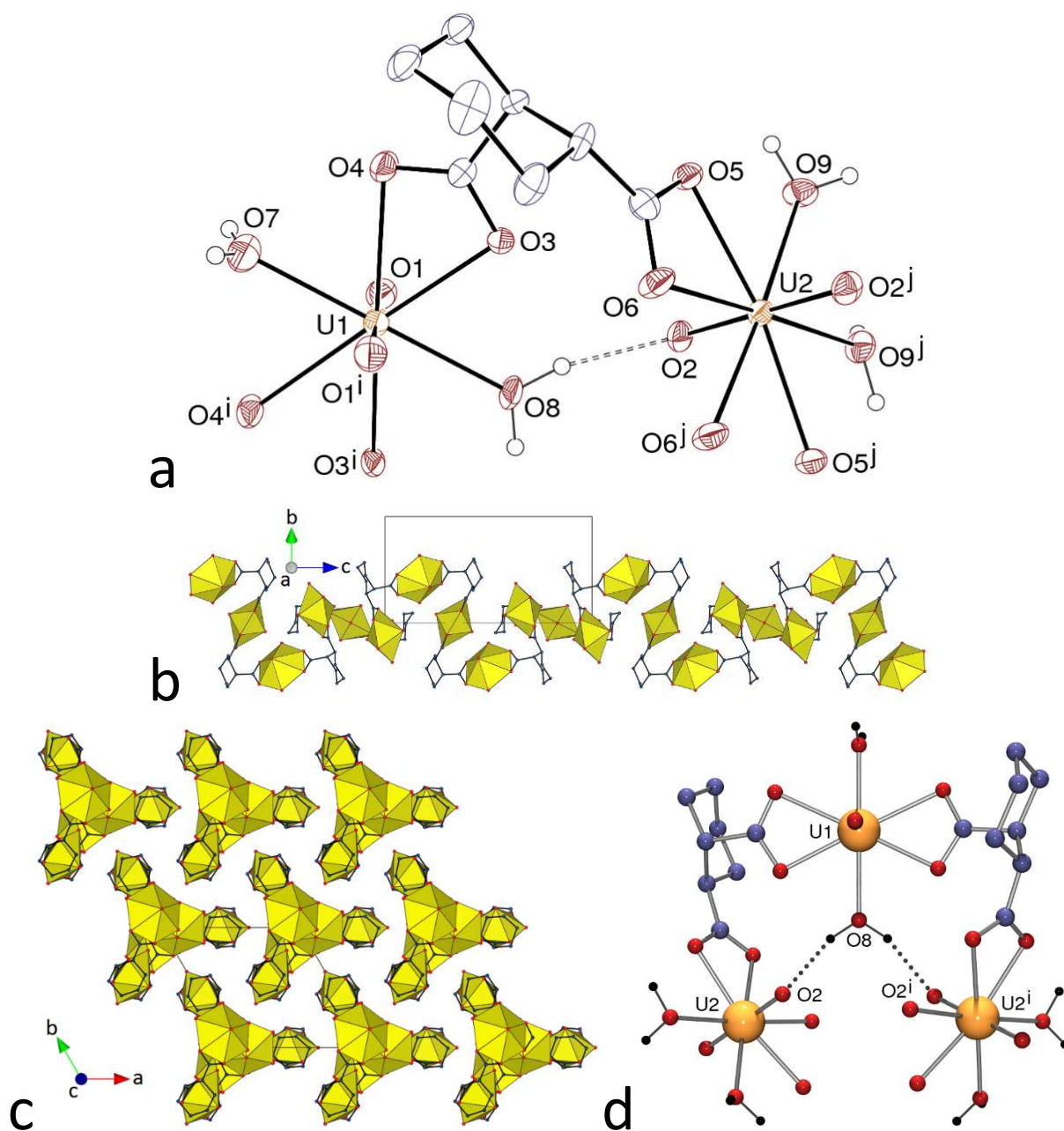
Figure 1. (a) View of compound 1. Displacement ellipsoids are drawn at the 40% probability level. Carbon-bound hydrogen atoms and solvent molecule are omitted, and the hydrogen bond is shown as a dashed line. Symmetry codes: i = y, x, 1 - z ; j = 2 - x, y - x + 1, 4/3 - z . (b) View of the 1D helical polymer. (c) Packing with chains viewed end-on. Uranium coordination polyhedra are colored yellow. (d) Intrachain hydrogen bonding (dotted lines).
