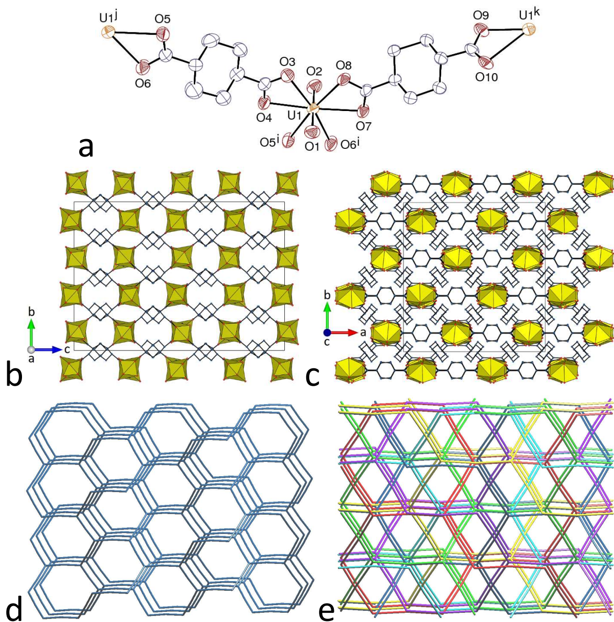
Figure 6. (a) View of compound 6. Displacement ellipsoids are drawn at the 30% probability level. Hydrogen atoms and counterions are omitted. Only one position of the disordered atoms is represented. Symmetry codes: i = 3/2 - x, y - 1/4, z + 1/4 ; j = 3/2 - x, y + 1/4, z - 1/4 ; k = 3/4 - x, 3/4 - y, z . (b) and (c) Two views of the 3D entangled framework. (d) Nodal representation of a single 3D assembly viewed down [010], with [100] horizontal. (e) Nodal representation of the sixfold interpenetrated net; same orientation as in d, but different scale.
