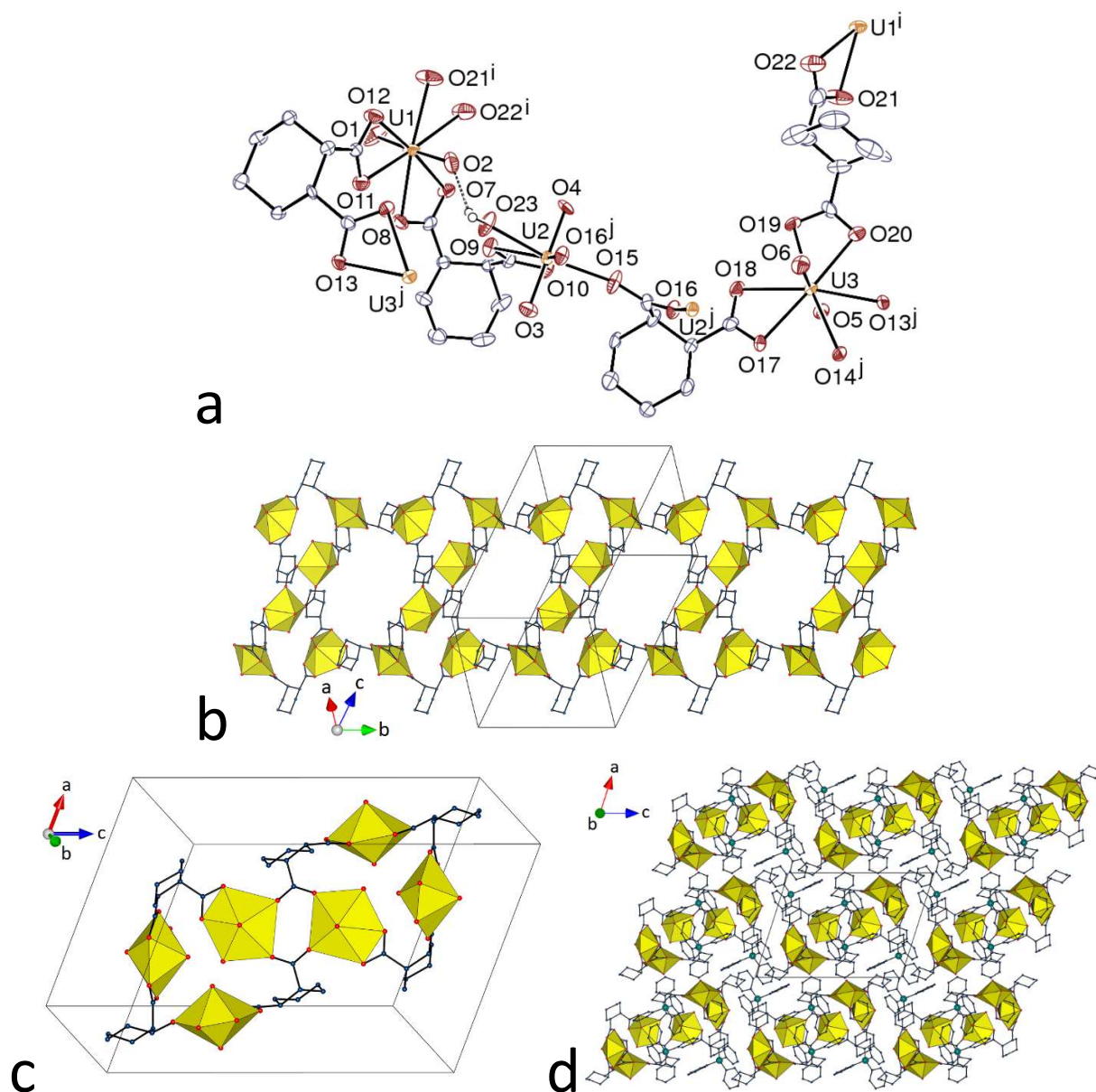
Figure 2. (a) View of compound 2 . Displacement ellipsoids are drawn at the 40% probability level. Carbon-bound hydrogen atoms, counterions and solvent molecules are omitted, and the hydrogen bond is shown as a dashed line. Symmetry codes: i = 1 - x, 2 - y, 1 - z ; j = 1 - x, 1 - y, 1 - z . (b) View of the 1D polymer. (c) View of the hexanuclear subunit. (d) Packing with chains viewed end-on; channels run obliquely, parallel to [101] .
