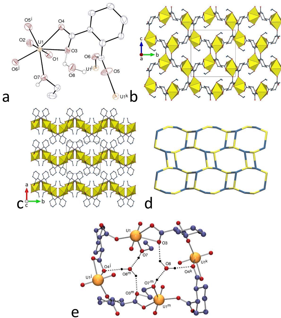
Figure 4. (a) View of compound 4. Displacement ellipsoids are drawn at the 40% probability level. Carbon-bound hydrogen atoms are omitted. Symmetry codes: i = x, 1/2 - y, z + 1/2 ; j = 1 - x, y - 1/2, 3/2 - z ; k = x, 1/2 - y, z - 1/2 ; l = 1 - x, y + 1/2, 3/2 - z . (b) View of the 2D assembly. (c) Packing with layers viewed edge-on. (d) Nodal representation of the 2D network (uranium, yellow; dicarboxylate ligand, dark blue; same orientation as in b). (e) Hydrogen bonding pattern; symmetry codes: as for a, and m = 1 - x, -y, 1 - z .
