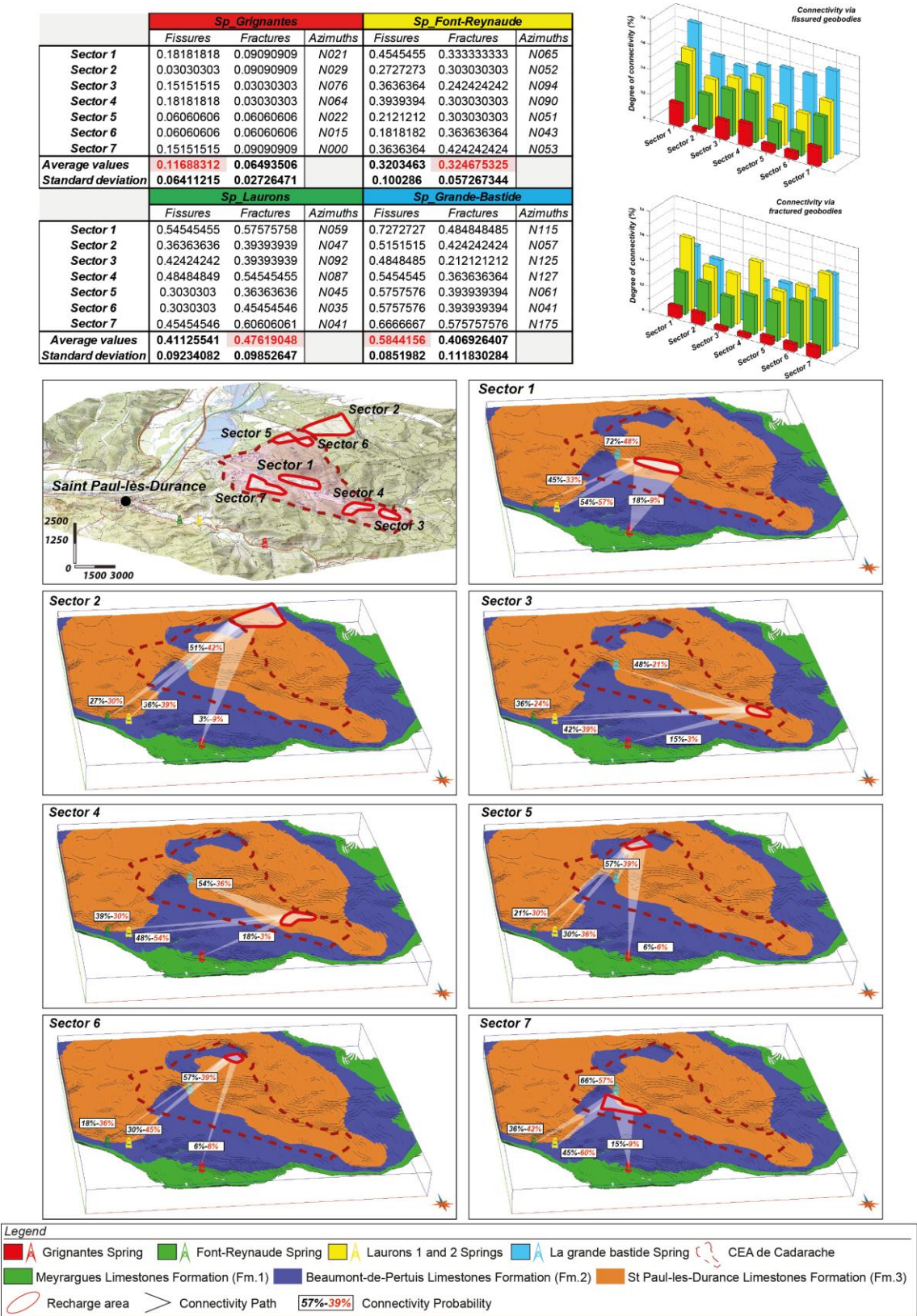
814 Figure 7 815 Bar diagram and map of static connectivity probability inside and between geobodies 816 containing major springs and seven sectors in the domain.
