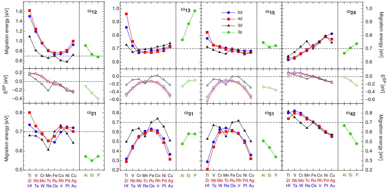
FIG. 5. DFT-computed iron migration barriers \omega_{ij} in the vicinity of a solute atom, according to the jump-frequency nomenclature of Fig. 1. The dashed lines mark the values in pure Fe ( \omega_{Fe} ). In the middle panels, the saddle-point contribution to each migration barrier, obtained by removing the initial-state binding energy and the pure-Fe vacancy migration barrier ( E_{ij}^{SP} = E_{ji}^{SP} ).
