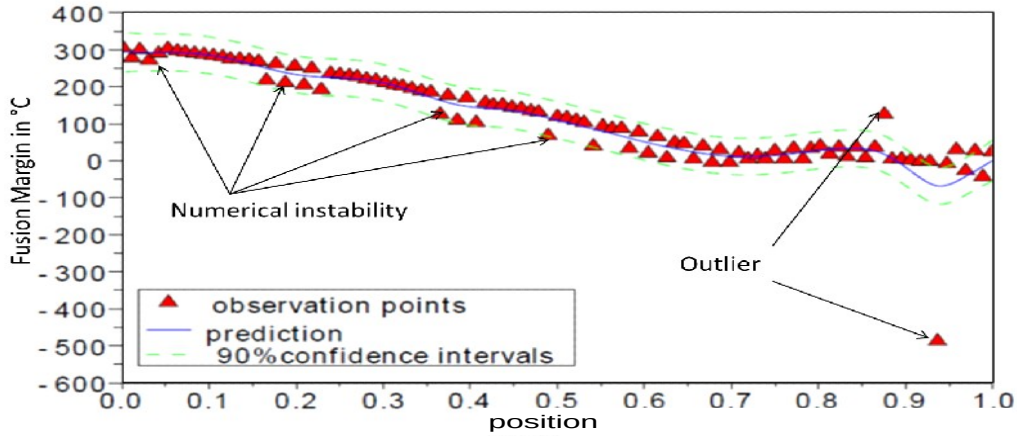
Figure 6: One-dimensional representation of the Germinal code function. We run 97 computations, which input points are located along a line segment, between two points \mathbf{a} and \mathbf{b} of the (normalized) input space [0, 1]^{11} . Input points are thus indexed by their position on the segment, where 0 corresponds to \mathbf{a} and 1 corresponds to \mathbf{b} . We observe a code instability, causing oscillations of the code response, that have no physical meaning but are caused by a preprocessing issue. We also show the prediction and 95% confidence intervals obtained with the Kriging estimated covariance parameters of Table II, where the support points of (7) and (8) correspond to these 97 computations. The output files of the two outlier computations contain the same warning as that described in Section 5.1.
