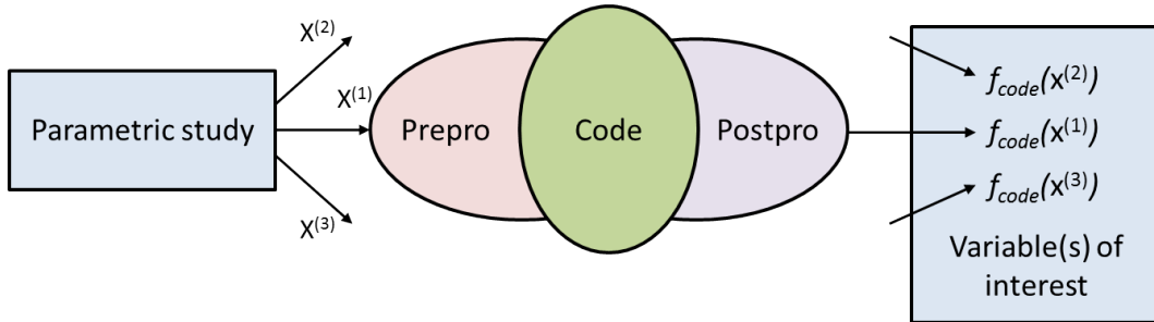
Figure 1: Illustration of the code manager. In a parametric study, all code simulations are characterized by a finite-dimensional vector \boldsymbol{x} of scalar parameters. The code manager first consists in a preprocessor, which generates code inputs from these parameters. After the simulation, the code manager incorporates a postprocessor, which checks the occurrence of computational failure and then condense the code output in some variables of interest.
