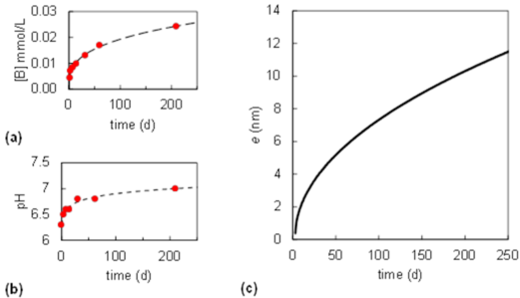
Figure 4: Evolutions of boron concentration (a) and pH (b) are derived from Hellmann et al. , 2015 data. Experimental data are fitted with power laws in order to calculate a continuous evolution of the thickness e of the diffusion zone versus time according to equation 9.
