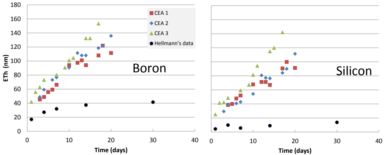
Figure 3: Equivalent thickness ETH of altered glass calculated from B (left) and Si (right). Here we compare results from a series of 3 experiments conducted at CEA in the 1990s with that obtained in Hellmann et al. (Hellmann et al., 2015). Both type of experiments were performed at 50^{\circ}\text{C} , low S/V ( 0.24\text{ cm}^{-1} for CEA's experiments and 0.1\text{ cm}^{-1} for Hellmann's experiment). Solution was stirred in CEA experiments and not for the Hellmann's experiment.
