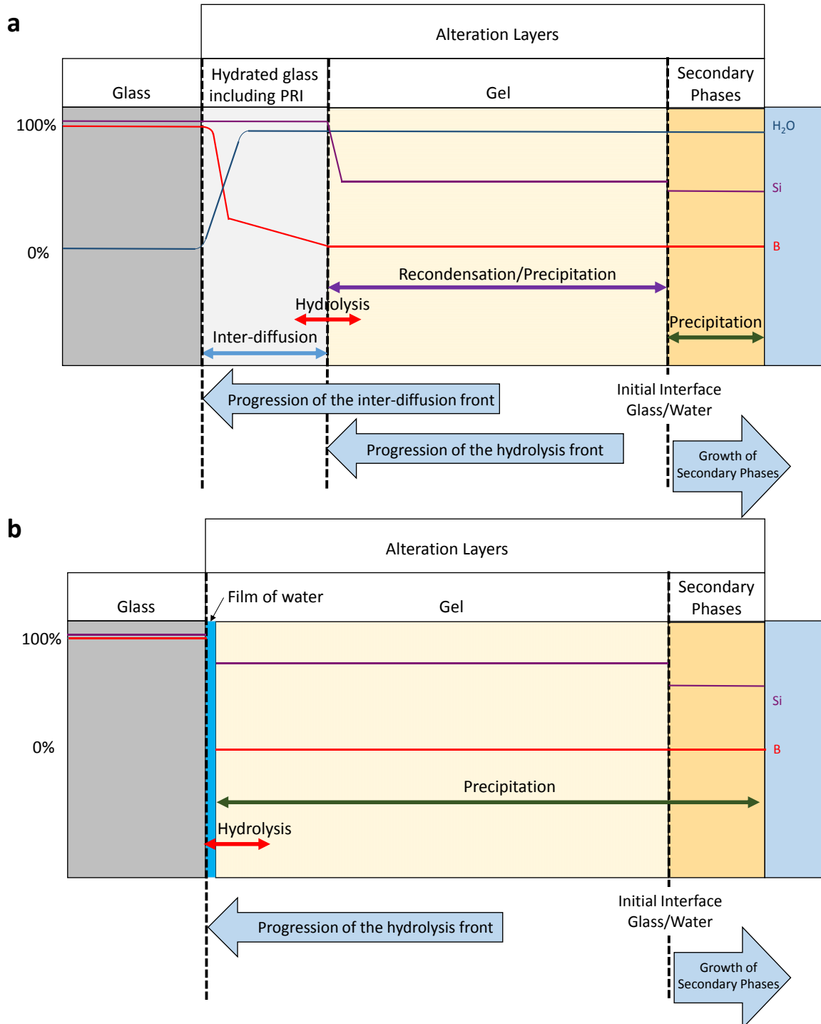
Figure 1: Sketch showing the layers formed during SON68 glass alteration: a) according to the classical theory including inter-diffusion and b) according to the interfacial dissolution-precipitation model. The thickness of each layer is indicative. It depends on the experimental conditions (temperature, pH, solution composition, flow rate).
