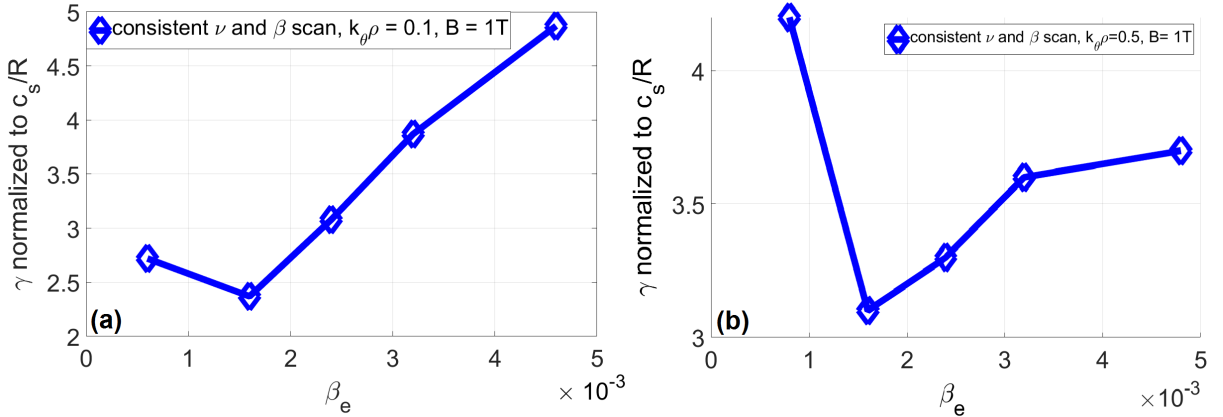
Figure 10. (a) Linear growth rate with GENE for k_\theta\rho = 0.1 , as a function of \beta_e = \beta/2 at \frac{\nu}{C_s/R} = 1.3 ( T_e = 50 eV) (b) Linear growth rate with GENE for k_\theta\rho = 0.5 , as a function of \beta_e = \beta/2 at \frac{\nu}{C_s/R} = 1.3 .
