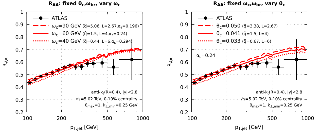
Figure 7. The effects of varying the medium parameters \hat{q} , L and \alpha_{s,\text{med}} in such a way to keep a constant value for \omega_{br} (the same as the central value in the right plot in Fig. 6, i.e. \omega_{br} = 3.46 GeV). Left: we vary \omega_c by \pm 50\% at fixed \theta_c . Right: we vary \theta_c^2 by \pm 50\% at fixed \omega_c .
