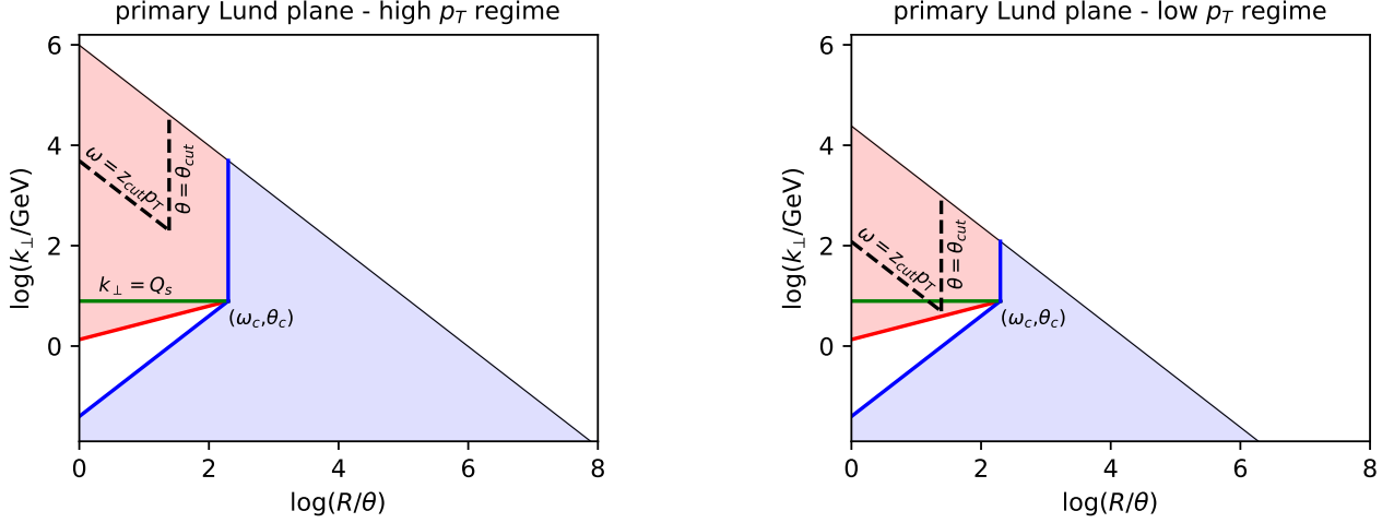
Figure 9. The kinematic regions in the Lund plane that are covered by the SD algorithm in the case of a high-energy jet ( z_{\text{cut}}p_T > \omega_c ) in the left figure and of a low-energy jet ( z_{\text{cut}}p_T < \omega_c ) in the right figure. As suggested by the pictorial representation in the right figure, the most interesting situation for “low-energy jets” is such that there is only little overlap between the kinematic region for SD and the phase-space for MIEs.
