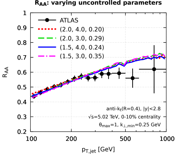
Figure 21. Left: our MC results for jet R_{AA} and for 4 sets of medium parameters which give quasi-identical predictions are compared to the ATLAS data [30] (black dots with error bars). Right: the MC predictions for the medium/vacuum ratio \mathcal{R}^{(\text{norm})}(z_g) of the self-normalised z_g distributions are presented in bins of p_T for the same 4 sets of medium parameters as in the left figure.
