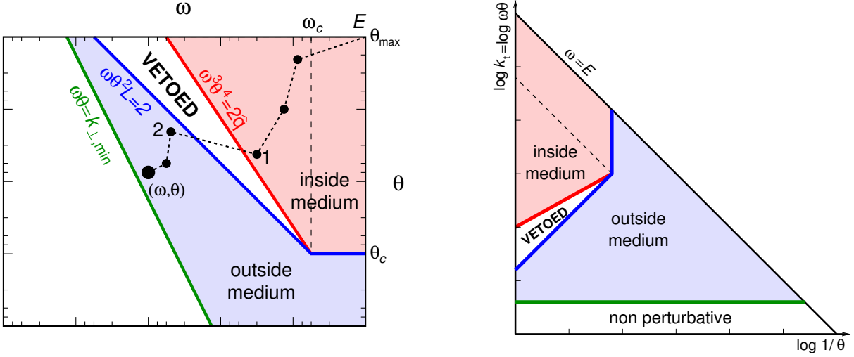
Figure 1. The phase-space for vacuum-like gluon emissions by a jet propagating through a dense QCD medium, in logarithmic units. In the left plot, the variables are the gluon energy \omega and its emission angle \theta . In the right plot, we rather use the relative transverse momentum k_{\perp} \simeq \omega\theta and the inverse of the angle 1/\theta .
