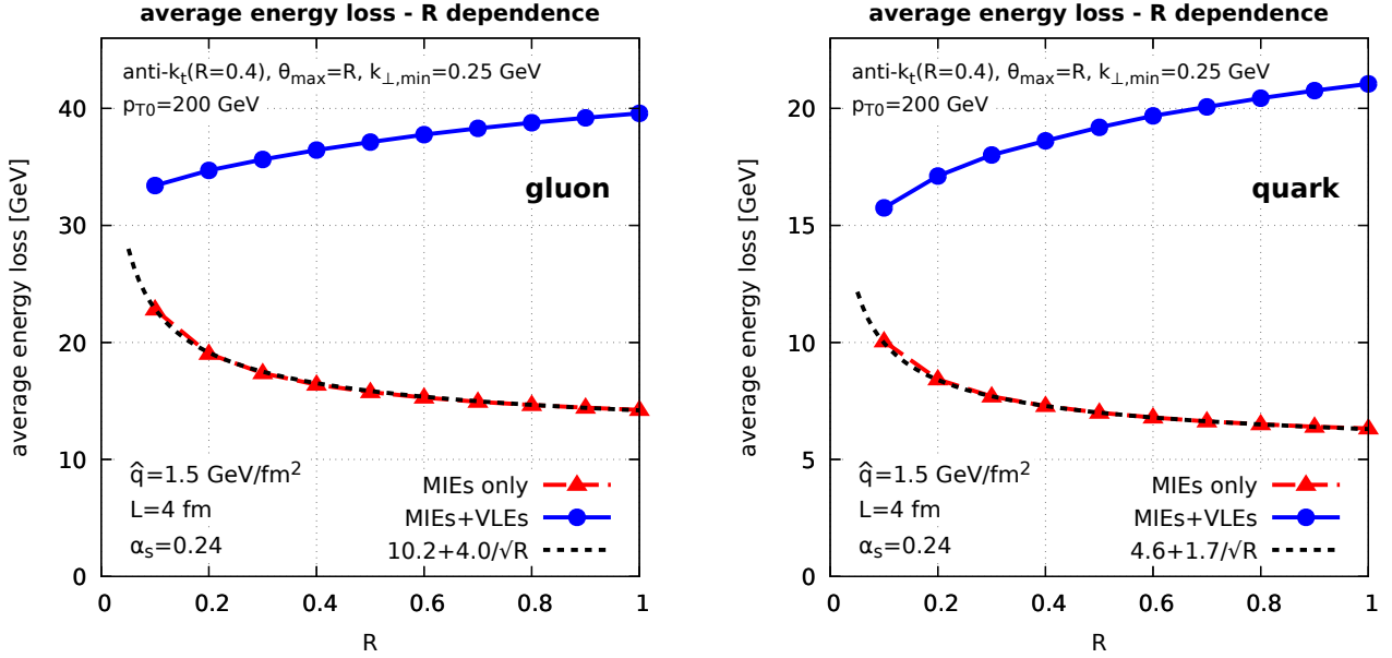
Figure 5. The MC results for the average energy loss by the jet are displayed as a function of the jet angular opening R , for the same choices as in Fig. 4. We also show in dashed line a fit (inspired by the theoretical estimate in Eq. (2.14)) for the jet built with MIEs alone.
