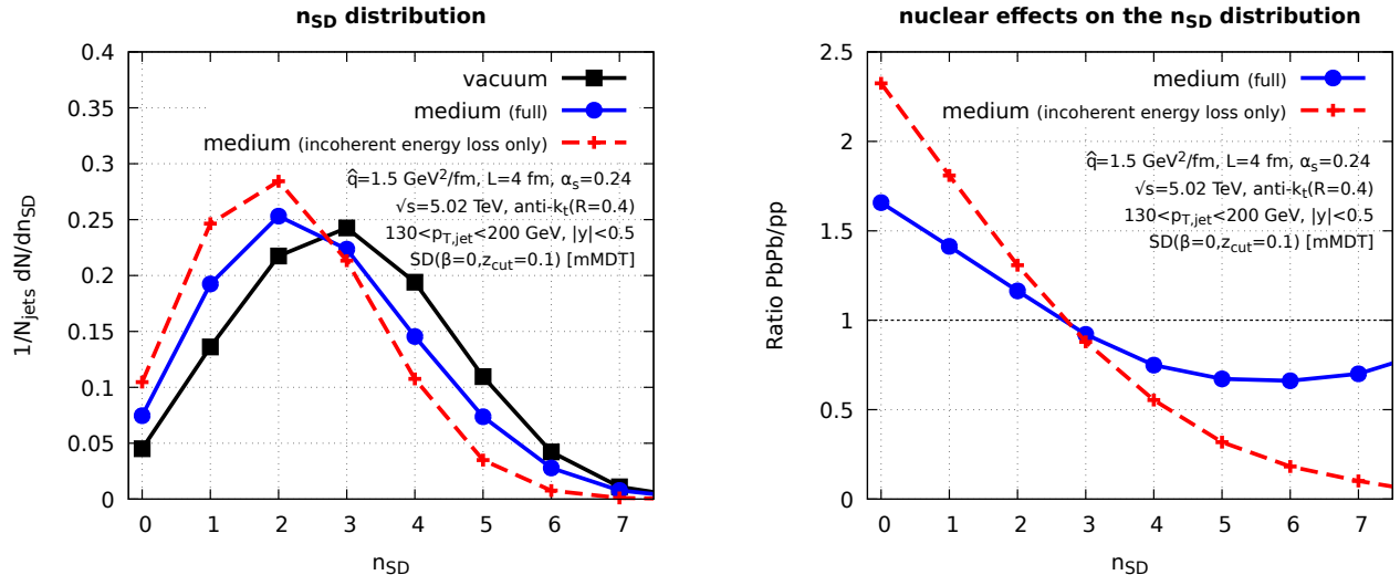
Figure 22. n_{SD} distributions emerging from our Monte Carlo simulations. Left: the distributions themselves, for the vacuum shower, for the full in-medium parton shower, and also for the case where the MIEs contribute only to the energy loss (but not directly to SD). Right: the medium/vacuum ratios.
