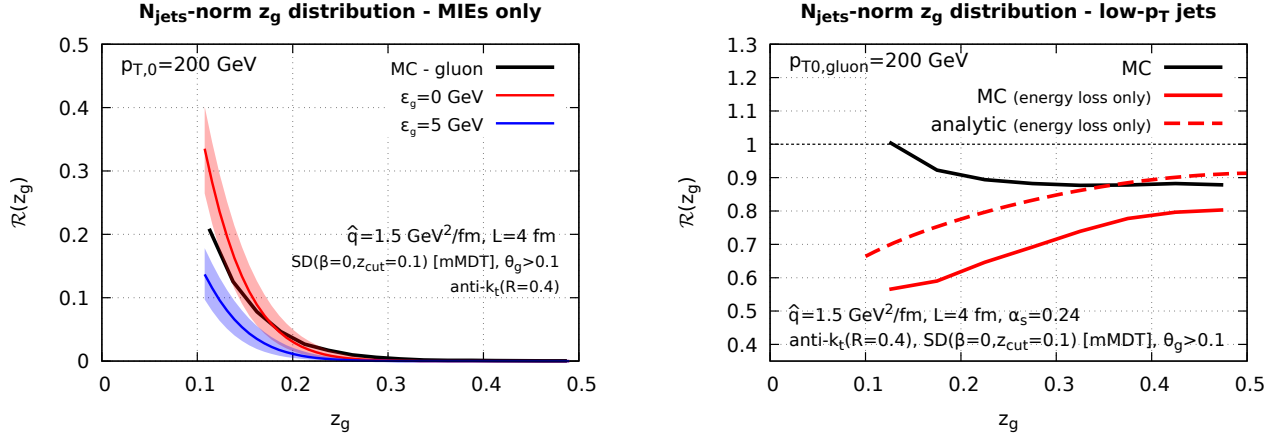
Figure 15. Separation of the nuclear effects on the z_g distribution of low-energy jets into a contribution due to the MIEs (left) and a contribution due to the VLEs with energy loss (right). Left: MIEs only (MC vs. analytic calculations). Right: Monte Carlo results for the full parton shower (black) vs. the case where only VLEs with energy loss are included (red). We also show an analytic result for the second case (dashed line).
