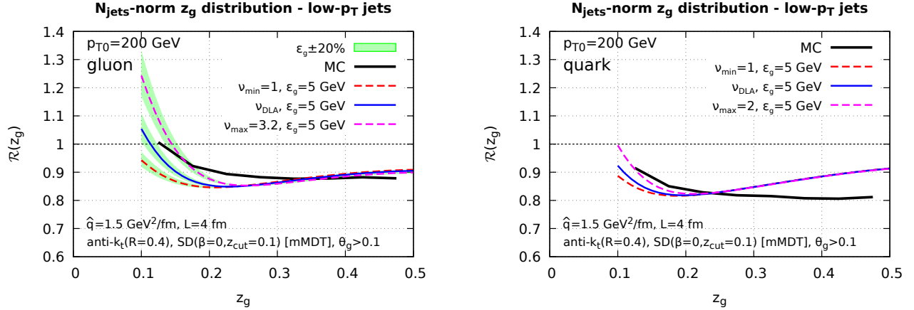
Figure 17. \mathcal{R}(z_g) for a leading parton (left: gluon, right: quark) with initial transverse momentum p_{T0} = 200 GeV. The Monte Carlo results are compared to analytic calculations corresponding to 3 different approximations for the number \nu of sources emitting MIEs (see the text for details).
