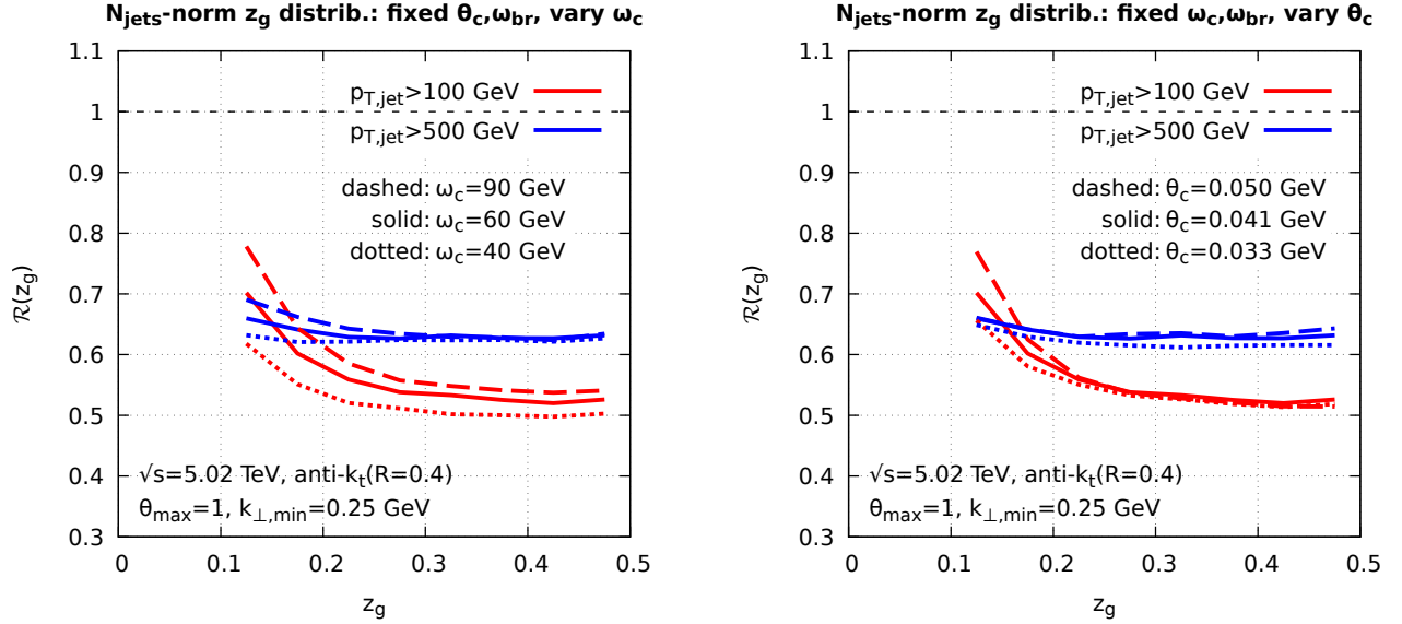
Figure 19. The effects of varying \hat{q} , L and \alpha_{s,\text{med}} keeping \omega_{\text{br}} = 3.46 GeV fixed at its central value (cf. the right plot of Fig. 6). Left: we vary \omega_c by \pm 50\% at fixed \theta_c . Right: we vary \theta_c^2 by \pm 50\% at fixed \omega_c .
