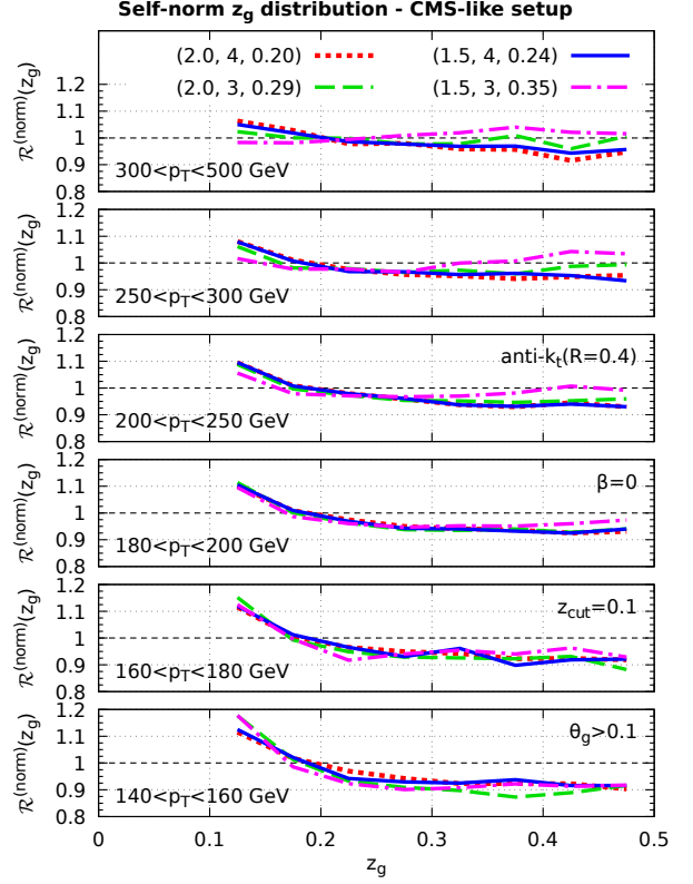
Figure 21. Left: our MC results for jet R_{AA} and for 4 sets of medium parameters which give quasi-identical predictions are compared to the ATLAS data [30] (black dots with error bars). Right: the MC predictions for the medium/vacuum ratio \mathcal{R}^{(\text{norm})}(z_g) of the self-normalised z_g distributions are presented in bins of p_T for the same 4 sets of medium parameters as in the left figure.
