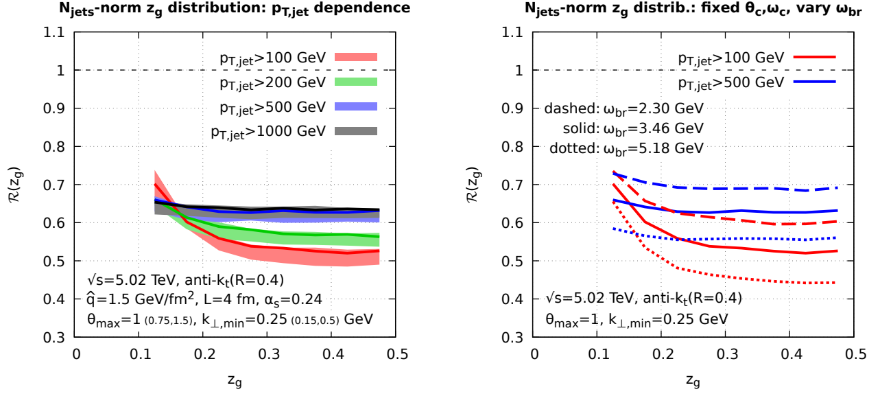
Figure 18. Our full MC predictions for the medium/vacuum ratio \mathcal{R}(z_g) of the N_{\text{jets}} -normalised z_g distributions, including the convolution with the initial jet spectrum. Left: the sensitivity of our results to changes in the kinematic cuts \theta_{\text{max}} and k_{\perp,\text{min}} . Right: the effect of varying \omega_{\text{br}} (by \pm 50\% ) at fixed values for \omega_c and \theta_c .
