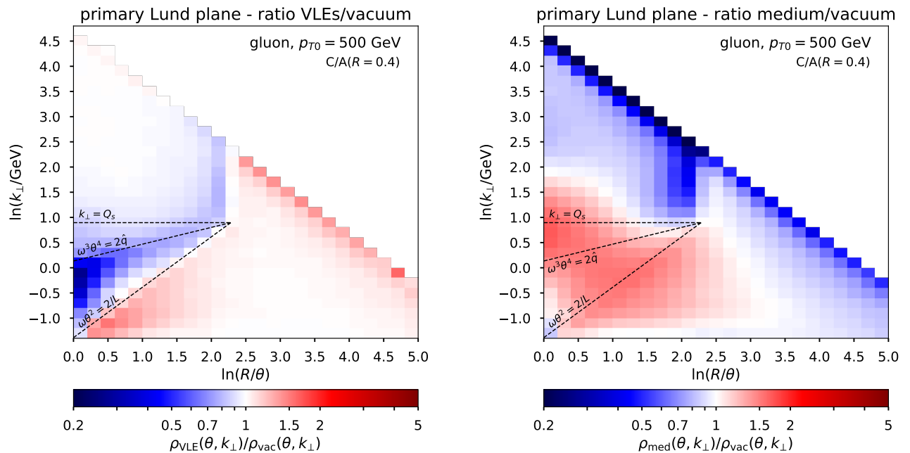
Figure 3. Effect of the medium on the primary Lund plane density \rho . The left plot show the ratio of the density obtained with VLEs, taking into account the kinematic constraints from the medium, to the vacuum reference. The right plot is the ratio of the full shower over the vacuum density.
