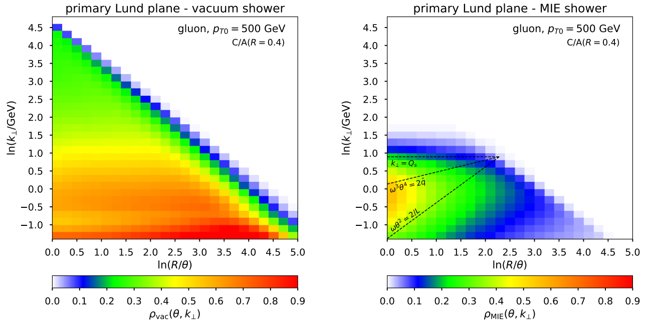
Figure 2. plot of the primary Lund plane density \rho for the two main showers in our Monte Carlo: the vacuum shower (left) and the medium-induced shower (right). In both cases, the shower is initiated by a 500 GeV gluon.
