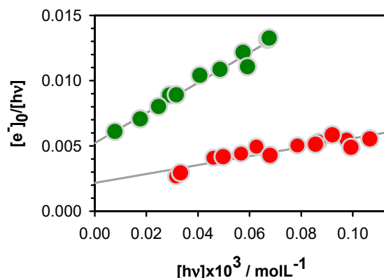
Figure 3. The ionization curves obtained for the duplex D (red) and the G-quadruplex TEL25/Na + (green); [e^-]_0 and [hv] denote, respectively, the zero-time concentration of hydrated ejected electrons and the concentration of absorbed photons per laser pulse. Experimental points (circles) are fitted with the linear model function [e^-]_0/[hv] = \phi_1 + \alpha[hv] (grey).
