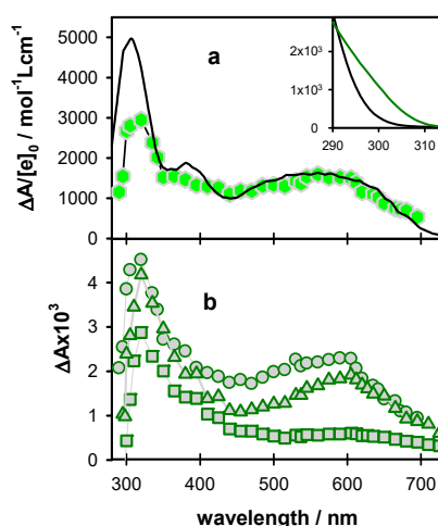
Figure 8. Differential absorption spectra determined for TEL25/Na + at 3 \mu s ((a); hexagons; average \Delta A from 2 to 4 \mu s), 5 \mu s ((b); circles; average \Delta A from 3 to 7 \mu s), 0.5 ms ((b); triangles; average \Delta A from 0.3 to 0.7 ms) and 10 ms ((b); squares; average \Delta A from 8 to 12 ms). The black line in (a) is a linear combination of the spectra corresponding to the radical cation (45%) [10] and the ( G-H2 ) • radical (55%) [16] of monomeric guanosine, considered with their \epsilon values. In the inset, the steady-state absorption spectra of dGMP (black) [62] and TEL25/Na + (green; see also Figure S5) are shown. The \epsilon is given per base.
