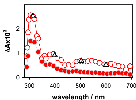
Figure 4. The differential absorption spectra determined for the duplex D at 5 \mu s (empty circles; average \Delta A from 3 to 7 \mu s) and 10 ms (full circles; average \Delta A from 8 to 12 ms). The triangles denote relative intensities of the 5 \mu s spectrum obtained using oxidation by SO_4^{\bullet-} [28].
