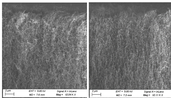
Fig. 7. SEM cross section of the top surface of VACNTs (sample G) before and after O 2 plasma etch.
