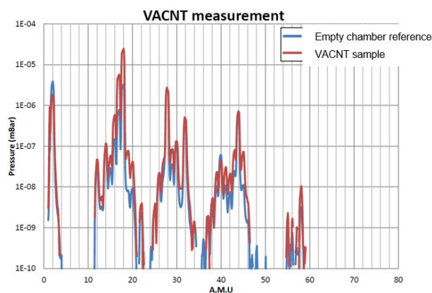
Fig. 8. Residual gas analysis spectra of the vacuum chamber with (red) and without (blue) VACNT sample.
