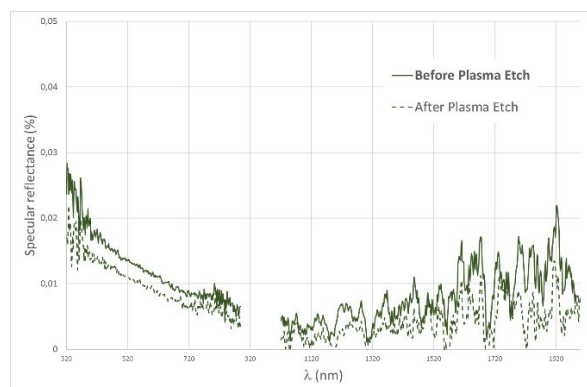
Fig. 6. Specular reflection spectra of VACNTs (sample G) before and after O 2 plasma etch.
