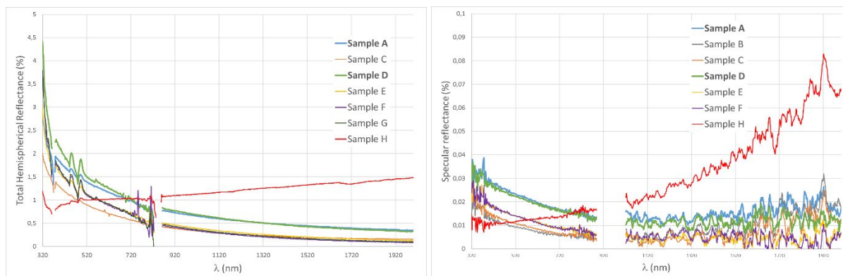
Fig. 3. Optical reflection spectra. The missing data have been intentionally removed due to low S/N ratio.
