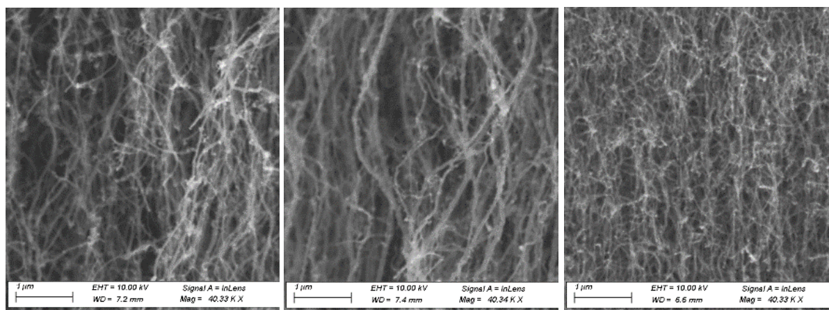
Fig. 2. SEM X-sections of samples D(left), A (center) and B (right).
