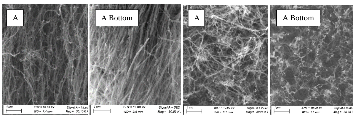
Fig. 4. SEM X-sections (left) and top views (right) of VACNTs before (A) and after (A Bottom) transfer on a plastic substrate.
