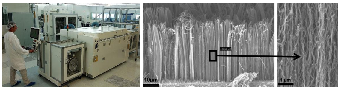
Fig. 1. Left: the roll-to-roll reactor; Center and right: SEM views of VACNTs grown in this reactor by atmospheric pressure aerosol assisted CCVD process on Al foil.
