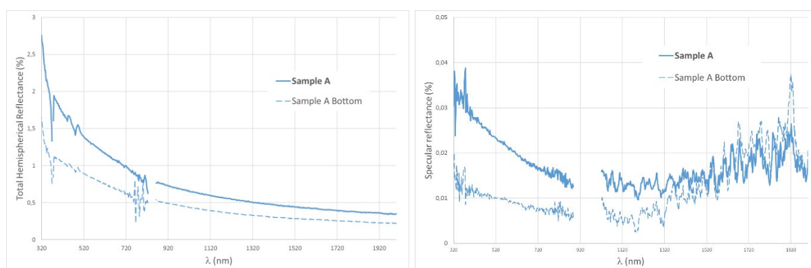
Fig. 5. Optical reflection spectra of VACNTs before (A) and after (A Bottom) transfer on a plastic substrate.
