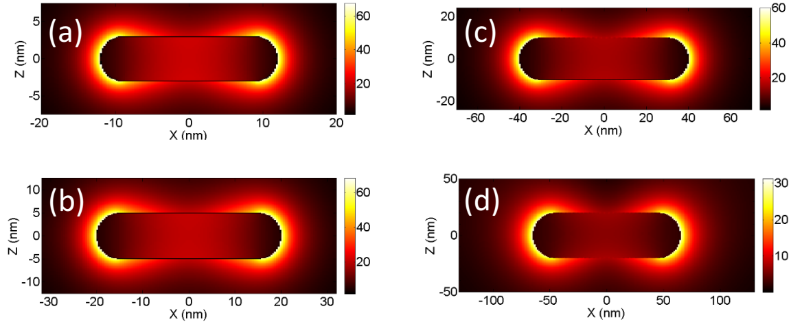
Figure SP5: Calculated electrostatic field enhancement map in intensity ( i.e. f^2_{loc-exc} ) for each GNR simulated with BEM : (a) 6 nm x 24 nm (b) 10 nm x 40 nm (c) 20 nm x 80 nm (d) 40 nm x 130 nm. The excitation wavelength is equal to the longitudinal resonance wavelength of each GNR (793 nm, 799 nm, 828 nm and 820 nm respectively) and the incident polarization is along the long axis of the GNR.
