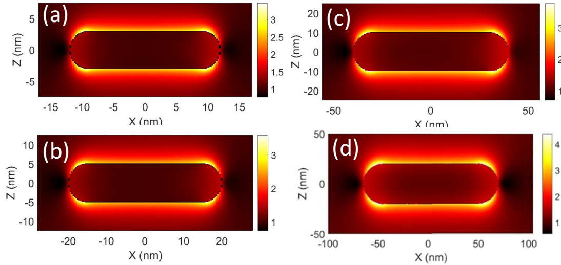
Figure SP6: Calculated electrostatic field enhancement map in intensity ( i.e. f^2_{loc-TPL} ) for each GNR simulated with BEM (a) 6 nm x 24 nm (b) 10 nm x 40 nm (c) 20 nm x 80 nm (d) 40 nm x 130 nm. The excitation wavelength is equal to the transverse maximum scattering wavelength of each GNR (522 nm, 522 nm, 522 nm and 534 nm respectively – see figure SP8) and the incident polarization is along the short axis of the GNR.
