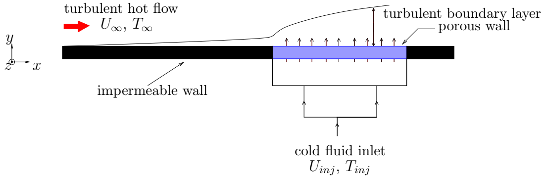
Fig. 2. General configuration.
