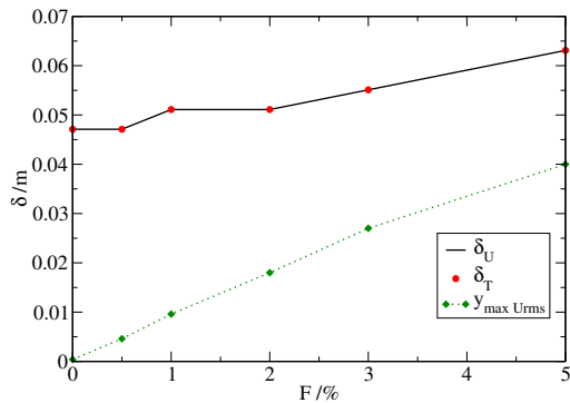
Fig. 10. Boundary layer thickness evolution with F .
