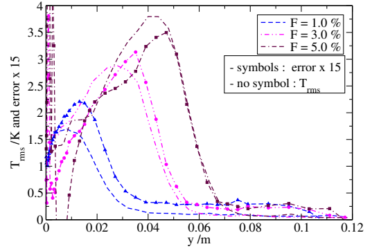
Fig. 6(b). Correlation between temperature fluctuations and error in velocity fluctuations estimation.
