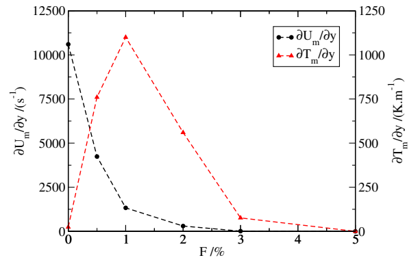
Fig. 9. Velocity and temperature gradients at the wall.
