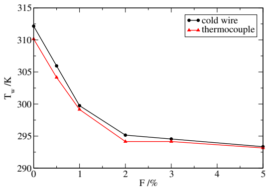
Fig. 8. Wall temperature measured with a thermocouple and by extrapolation from cold wire.
