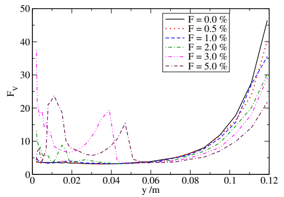
Fig. 20. Flatness factor F_V .
