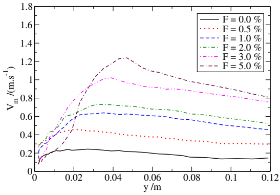
Fig. 13. Mean vertical velocity.
