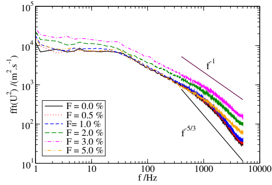
Fig. 23. Velocity spectrum at y = 31 \text{ mm} .
