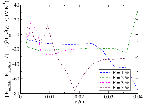
Fig. 7(b). Thermoelectrical effect on the vertical cold wire.
