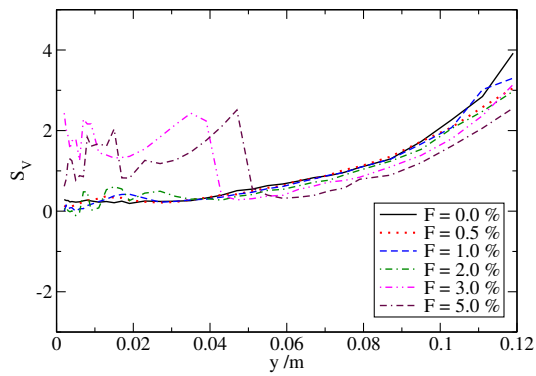
Fig. 19. Skewness factor S_V .
