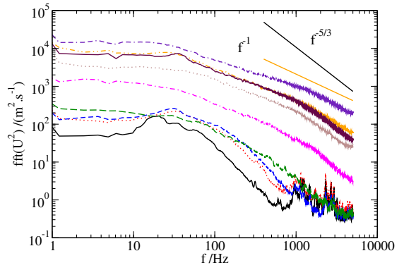
Fig. 25. Velocity spectrum for F = 5.0\% .
