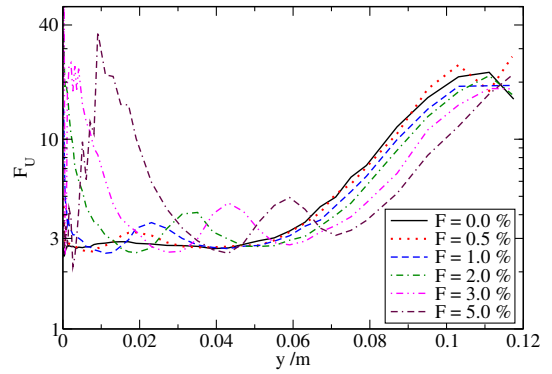
Fig. 18. Flatness factor F_U .
