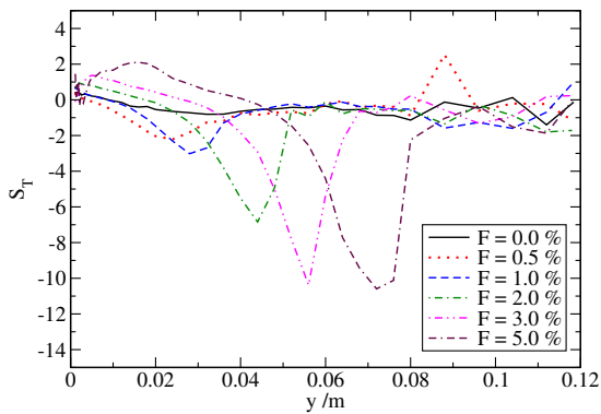
Fig. 21. Skewness factor S_T .
