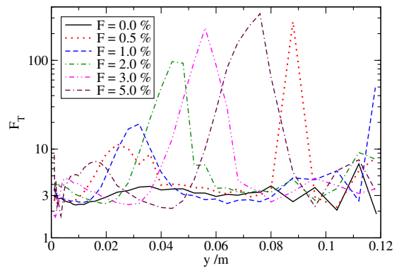
Fig. 22. Flatness factor F_T .
