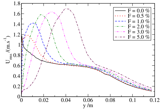
Fig. 12. Longitudinal velocity fluctuations.
