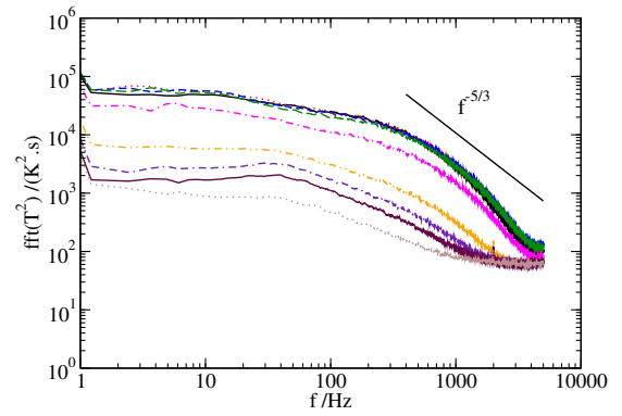
Fig. 27. Temperature spectrum for F = 5.0\% .
