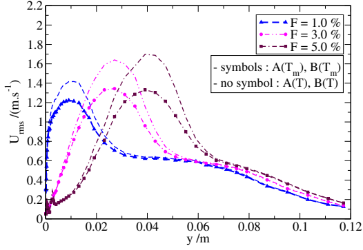
Fig. 6(a). Velocity fluctuations with instantaneous or mean temperature correction for A and B .
