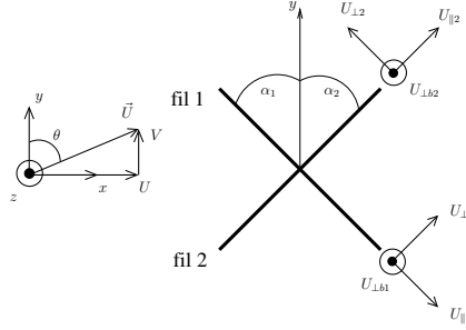
Fig. 5. Wires and laboratory referentials.
