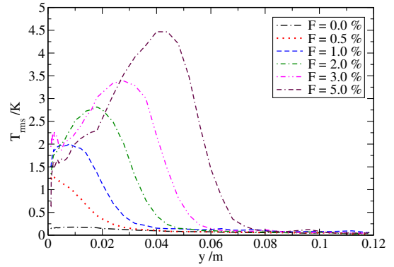
Fig. 16. Temperature fluctuations.
