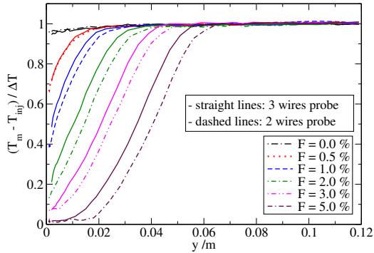
Fig. 7(a). Mean temperature profiles with the 2 and 3-wire probes.
