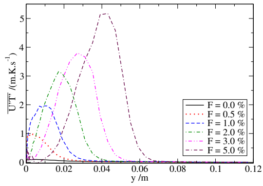
Fig. 28. \overline{U'T'} correlation.
