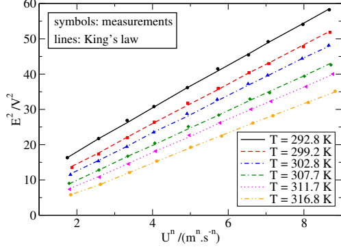
Fig. 4(a). Hot wires calibration (symbols : measurements, lines : King's law).
