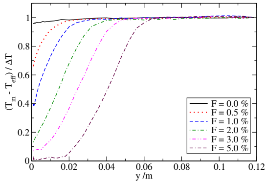
Fig. 15. Mean temperature.
