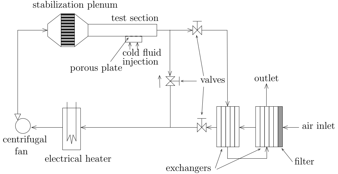
Fig. 1. Heated wind tunnel.
