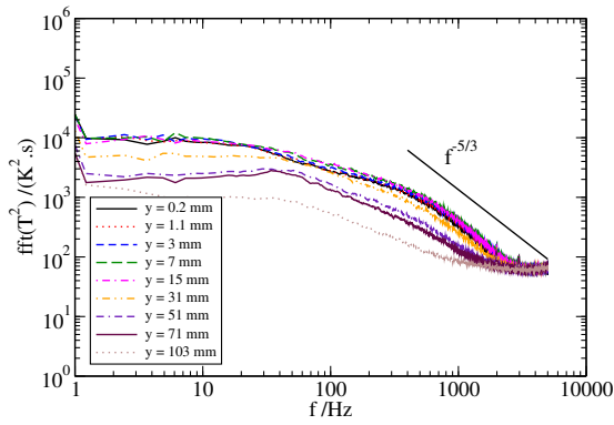
Fig. 26. Temperature spectrum for F = 0.0\% .
