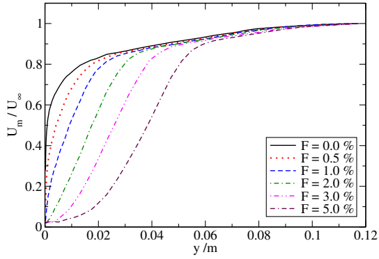
Fig. 11. Mean longitudinal velocity.
