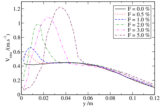
Fig. 14. Vertical velocity fluctuations.
