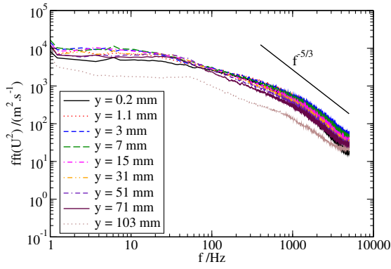
Fig. 24. Velocity spectrum for F = 0.0\% .
