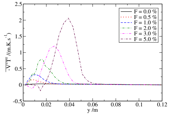
Fig. 29. -\overline{V'T'} correlation.
