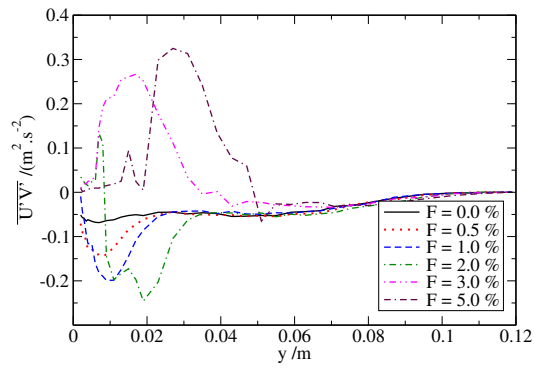
Fig. 30. \overline{U'V'} correlation.
