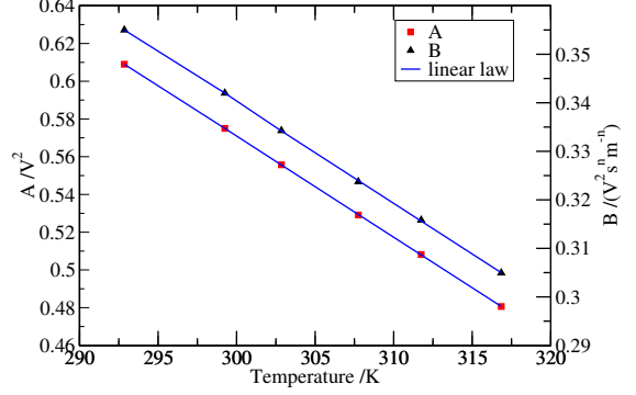
Fig. 4(b). A and B coefficients evolution with the temperature ( n = 0.46 ).
