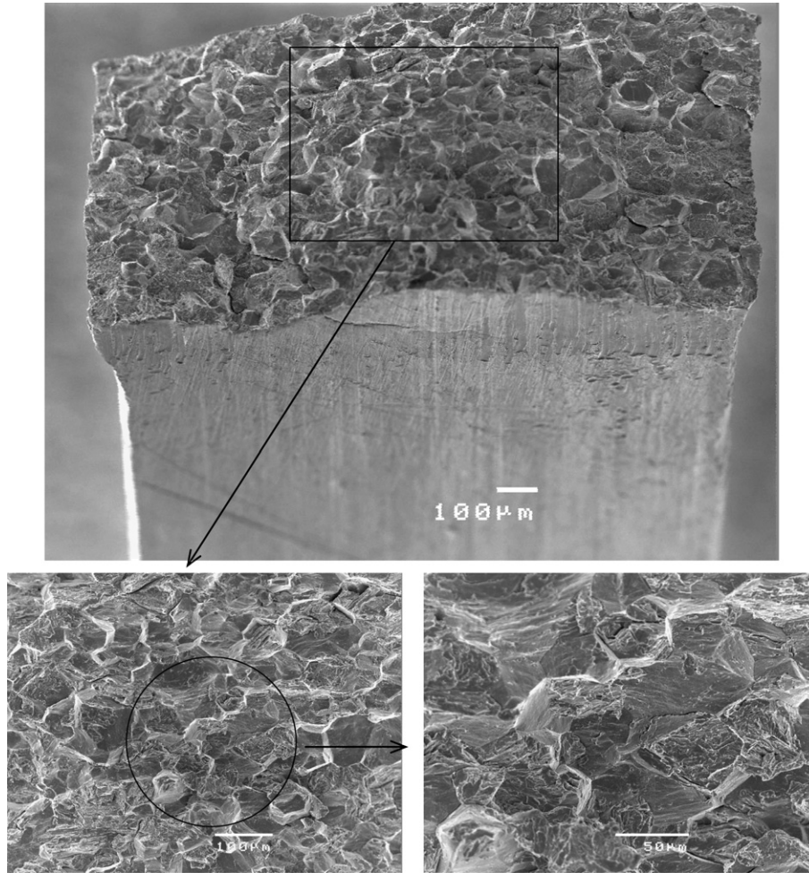
Fig. 18. SEM micrographs showing the fracture surface of EM10 specimen G31 ('L' type) irradiated to 17.9 dpa and tested at room temperature.
