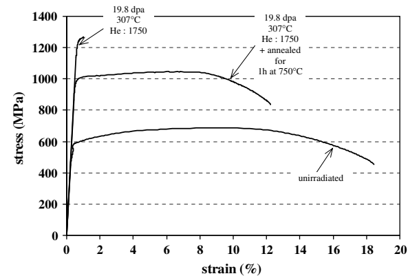
Fig. 3. Tensile curve measured at room temperature for an EM10 specimen (S geometry) annealed following irradiation compared to the 'as-irradiated' curve.
