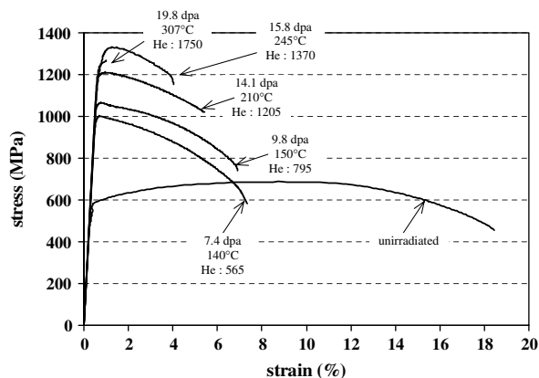
Fig. 2. Examples of stress/strain curves for EM10 'S' type specimens tested at room temperature. For each curve, the dose, helium content in appm and average temperature (as defined in Table 2) are indicated.
