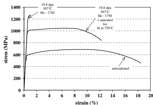
Fig. 3. Tensile curve measured at room temperature for an EM10 specimen (S geometry) annealed following irradiation compared to the 'as-irradiated' curve.
