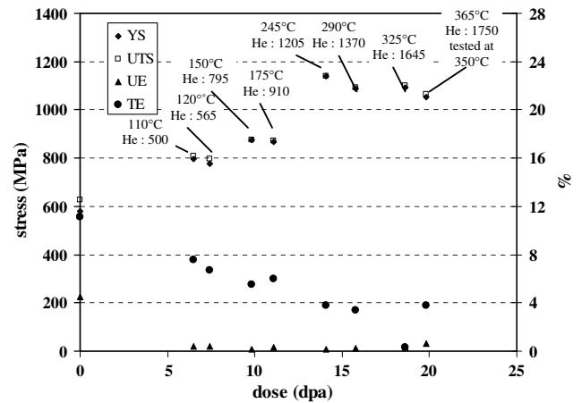
Fig. 13. Tensile properties (YS: yield stress; UTE: ultimate tensile strength; UE: uniform elongation; TE: total elongation) as a function of dose measured at 250 °C on EM10 tensile specimens ('S' type). For each set of data points, Helium content and average irradiation temperature are indicated (in some cases, two samples with identical doses and different temperatures were tested). The data points for one sample irradiated at the maximum dose and tested at 350 °C are also plotted.
