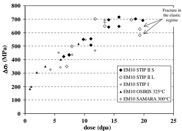
Fig. 26. Increase in yield stress as a function of dose for the EM10 specimens in the Normalised and Tempered metallurgical condition after exposure in a spallation environment (STIP II and STIP I [3] irradiations) or with fission neutrons (irradiations in the OSIRIS [4] and SM2 [5] thermal reactors). The data points indicated by arrows were calculated as the difference between the fracture stress following irradiation and the yield stress of the unirradiated steel since the specimens broke in the elastic regime.
