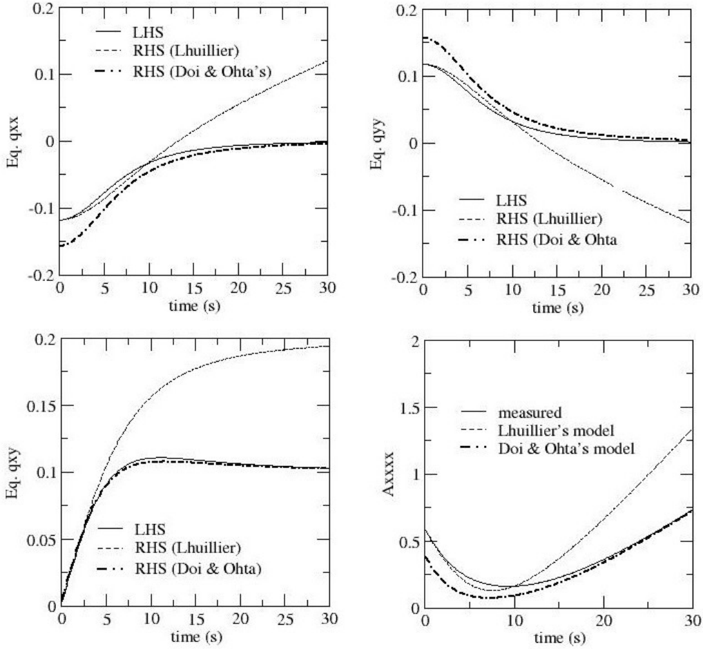
Fig. 11: Comparison of Lhuillier's model (97) to the model (92) on the elongation and rotation case. Comparison of the LHS and RHS of the model equations (118) for the quantities q_{xx} , q_{xy} and q_{yy} . Comparison of the measured and modeled quantity A_{xxxx} .
