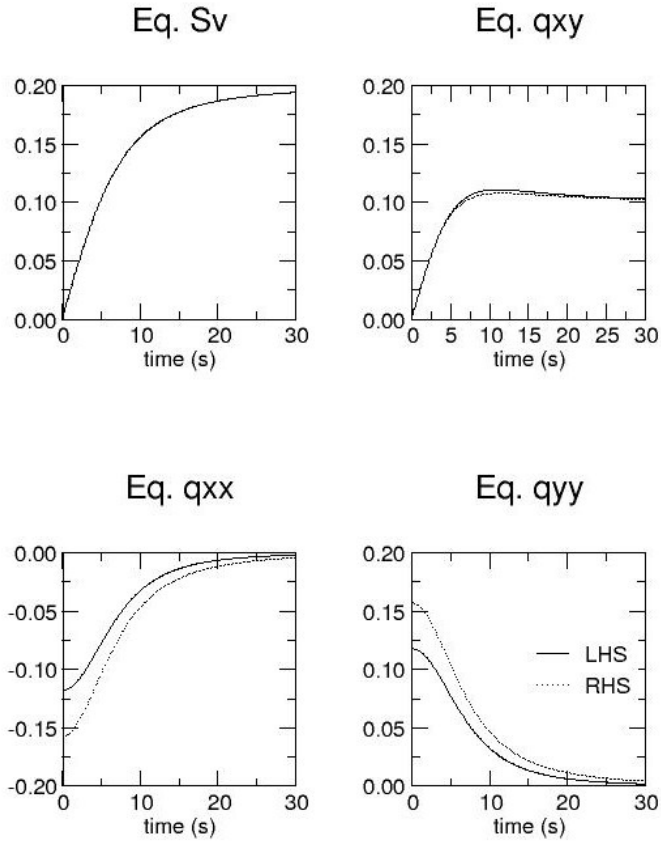
Fig. 9: Comparison of the LHS and RHS of the model equations (117) (elongation and rotation)
