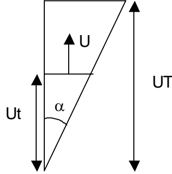
Fig. 1: A plane surface moving in a sector
