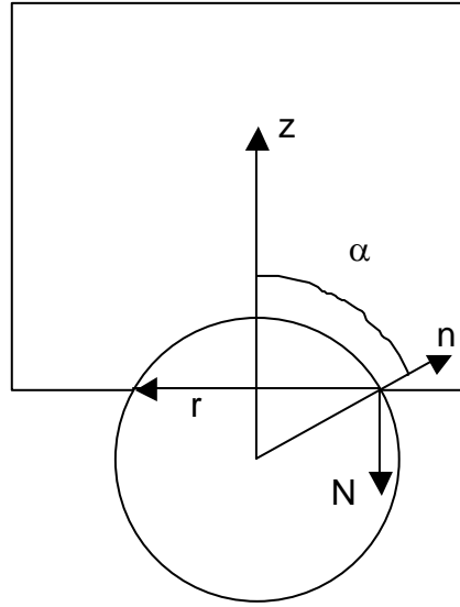
Fig. B: Definition of the \alpha angle
