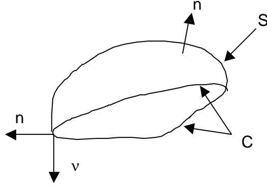
Fig. 3: An open surface evolving freely in space
