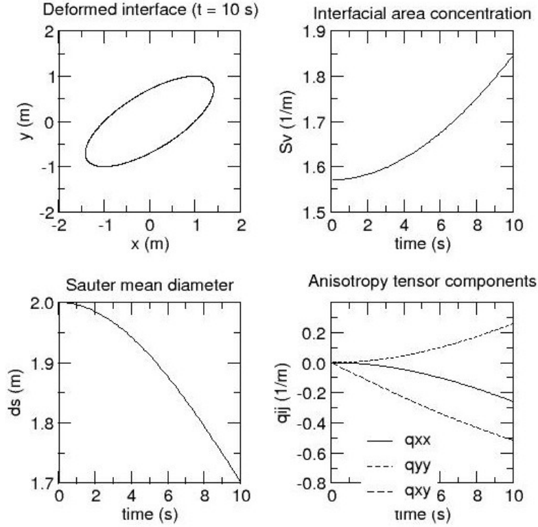
Fig. 5: Sketch of the deformed interface at the end of the calculation and time evolution of the volume-averaged quantities S_V , d_S and q_{ij} (simple shear)
