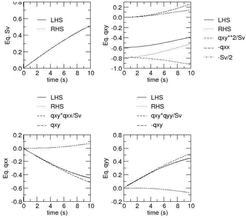
Fig. 6: Comparison of the LHS and RHS of the model equations (114) together with the different contributions in their RHS (simple shear)
