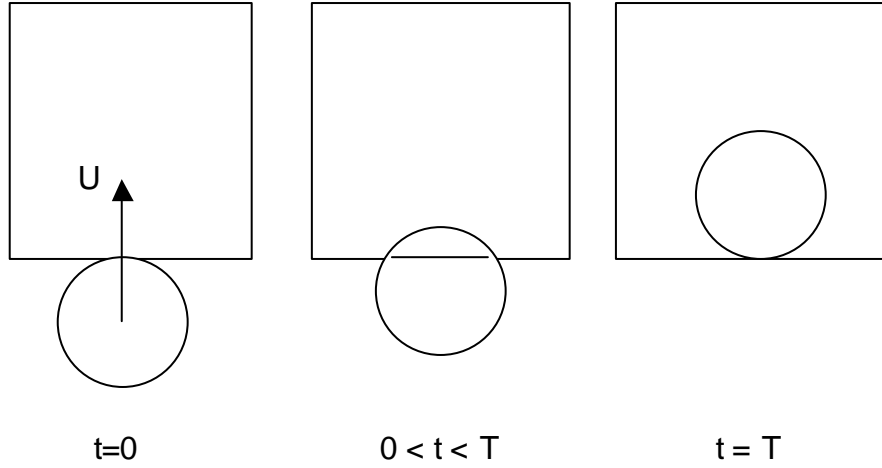
Fig. 2: A spherical bubble entering in a cubic box
