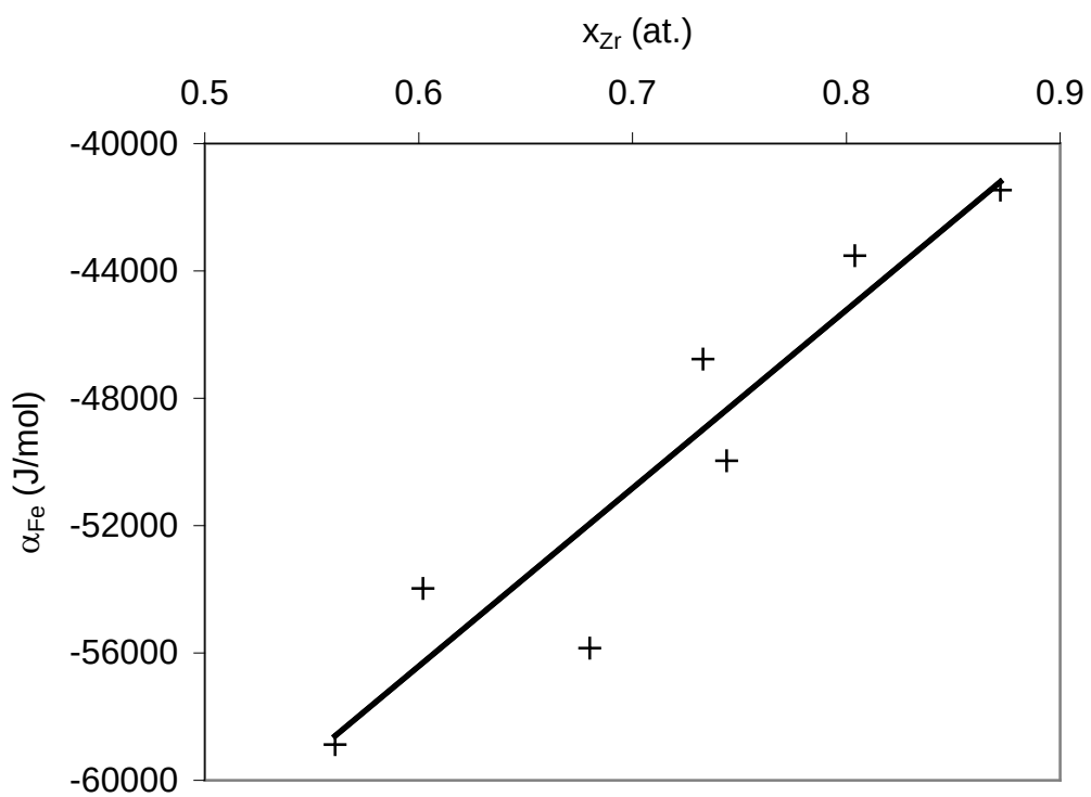
Figure 6. The function \alpha_{Fe} = f(x_{Zr}) at T = 1700 \text{ K}
