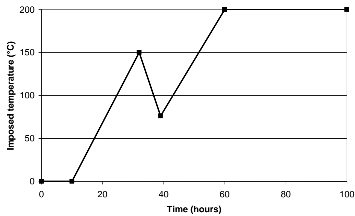
Figure 16. Thermal loading
