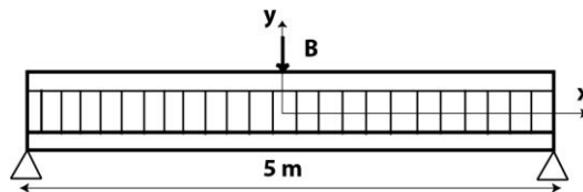
Figure 9. Geometry of three point bending beam.
