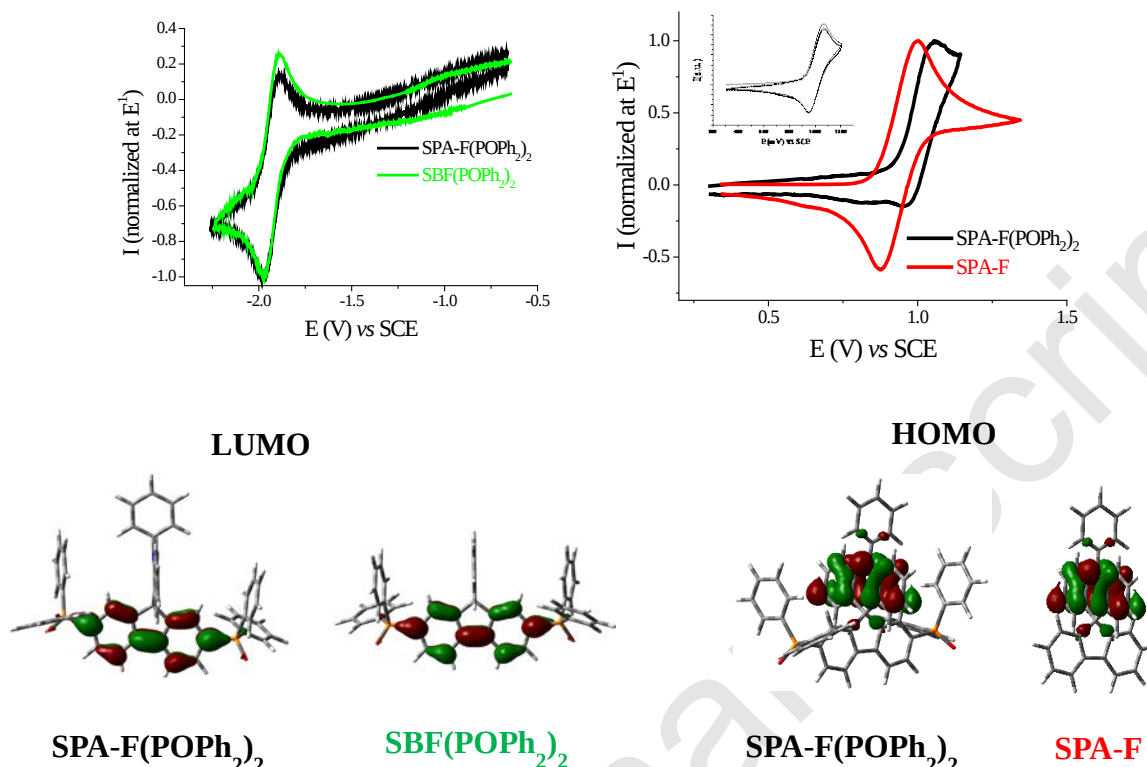
Figure 1. Top. Normalized cyclic voltammograms of SPA-F(POPh 2 ) 2 (black lines), SBF(POPh 2 ) 2 (green lines) and SPA-F (red lines) in the cathodic (left, DMF + Bu 4 PF 6 0.1 M) or the anodic (right, CH 2 Cl 2 + Bu 4 NPF 6 0.2 M) range. Sweep-rate of 100 mV·s -1 , platinum disk (diameter 1 mm) working electrode. Inset in oxidation: first oxidation of SPA-F(POPh 2 ) 2 at 1 V/s. Bottom: Frontier molecular orbitals obtained by DFT (B3LYP 6-31+G(d,p)).
