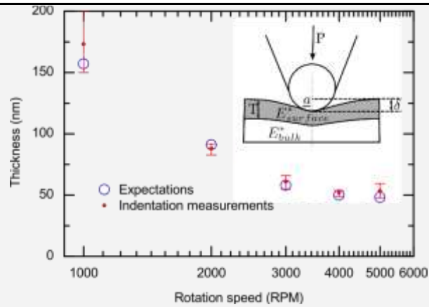
Figure 2. Thicknesses measured with indentation models and expectations. Inset. Hertzian indentation of a bilayer.
