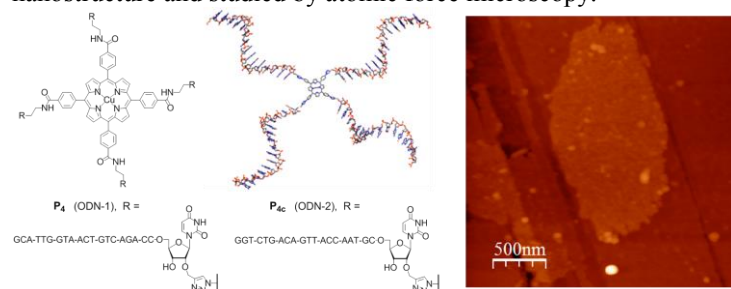
Figure. Representation of the tetra-adduct porphyrin-oligonucleotide hybrids and AFM image of a 2D nanostructure.
