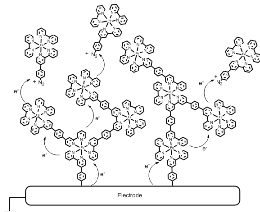
Scheme 1. Scheme of an electrografting of a diazonium salt of TBPFediazonium salt on a gold electrode.
