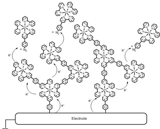
Scheme 1. Scheme of an electrografting of a diazonium salt of TBPF on a gold electrode.
