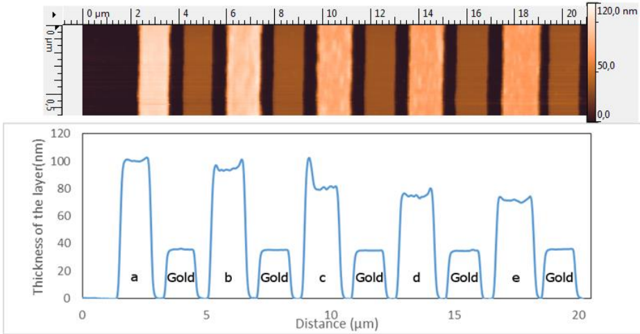
Figure 1. AFM image of gold electrodes grafted in different conditions with a TBPF diazonium salt (up) and its corresponding profile (down). The electrodes a, b, c, d and e are grafted while the gold electrodes are used as a height reference.
