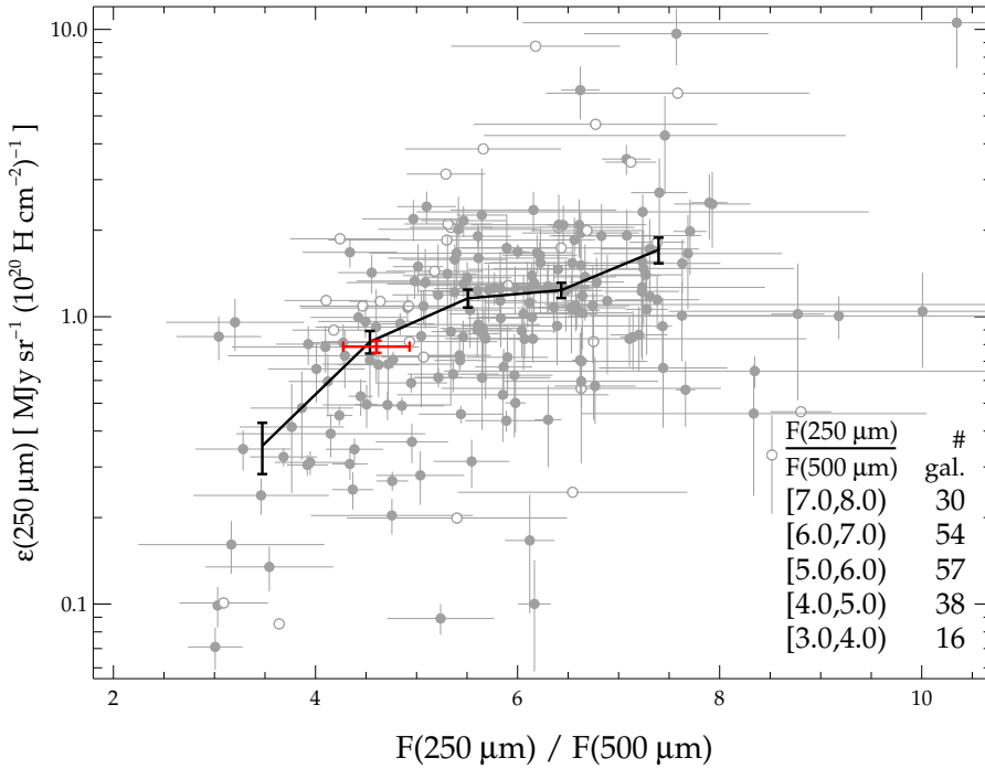
Fig. 2. Emissivity \epsilon(250 \mu\text{m}) as a function of the F(250 \mu\text{m})/F(500 \mu\text{m}) ratio. When data on the abscissa (and/or ordinate) are estimated at a level below 2\sigma , the x (and/or y ) error is omitted and an open symbol is used. The red error bar shows the MW estimate from HeVICS. The mean of \epsilon(250 \mu\text{m}) and its standard deviation for five bins in F(250 \mu\text{m})/F(500 \mu\text{m}) is shown by the black error bars (connected by a solid line). The F(250 \mu\text{m})/F(500 \mu\text{m}) range and the number of galaxies is given for each bin.
