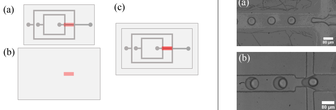
Left : Schematic representation illustrating the principle of the technique, (a) chip and (b) flat PDMS with the parts that need to remain hydrophobic protected by ink (in red), (c) the chip after bonding - Right: Use of a patterned chip to form double emulsion, (a) formation of water-in-oil droplets without wetting and (b) formation of water-in-oil-in-water droplets.
