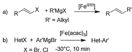
Scheme 1. Representative examples of Fe-catalyzed C—C cross-couplings.
