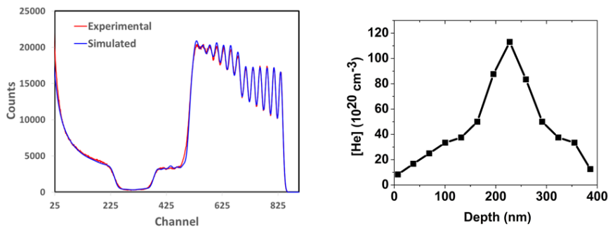
RBS spectrum of a Cr/Ta multilayer coated sample after heavy ion irradiation (left) and helium distribution after 2 \times 10^{17} \text{ cm}^{-2} implantation (right)
