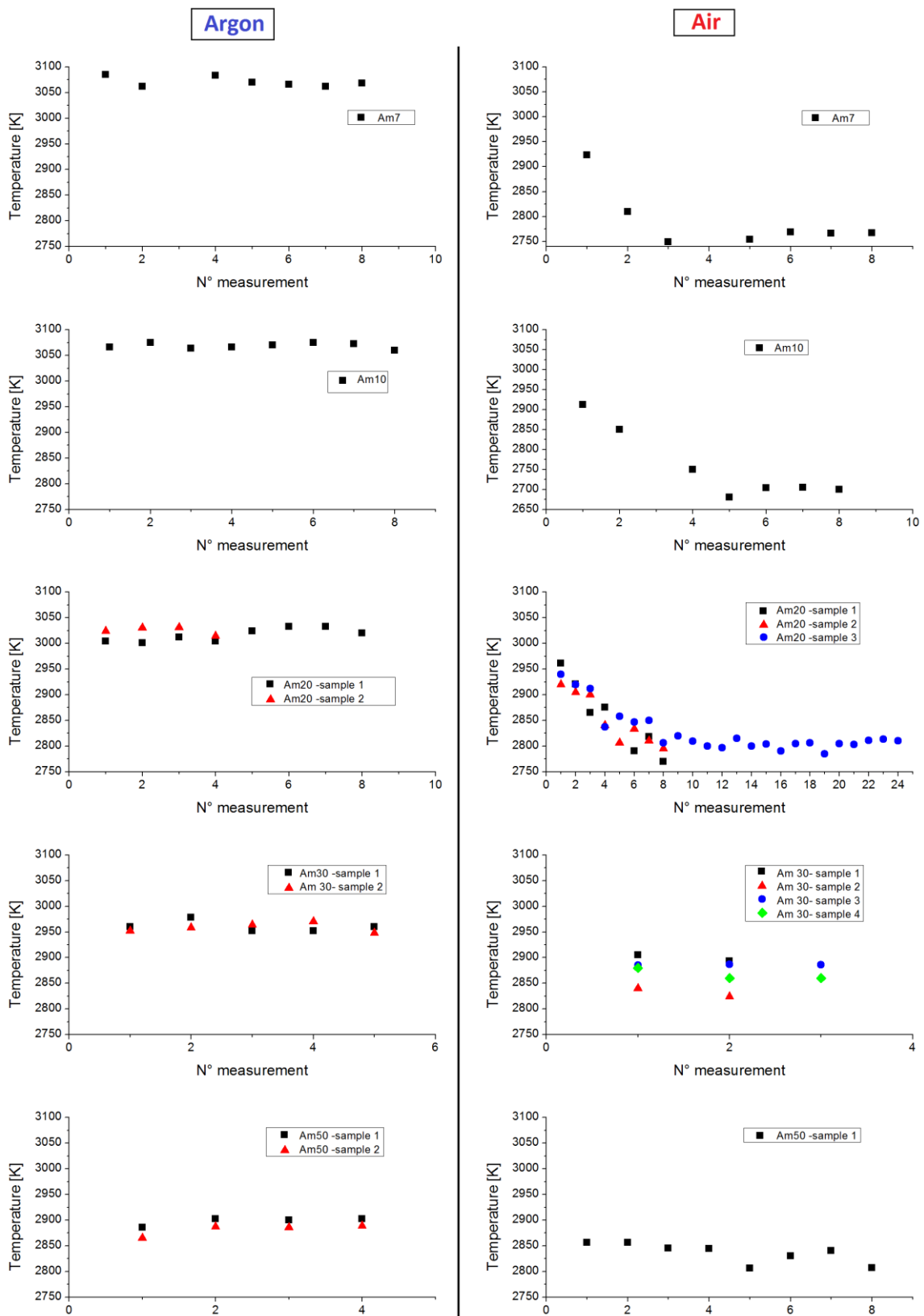
Figure 2. Solidus temperature results obtained in successive measurements in Ar and air.
