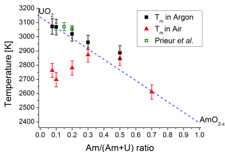
Figure 3. Melting ( solidus ) temperatures as a function of the initial Am/(Am+U) ratio of the samples. The results of this work are compared to the data reported in the literature for UO_2 , AmO_{2-x} and (U, Am)O_2 oxides with Am/(Am+U)=0.10, 0.15, 0.20 .
