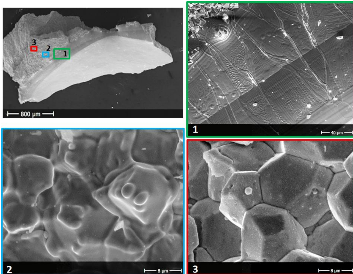
Figure 4. SEM images acquired on the Am50 sample melted in argon.
