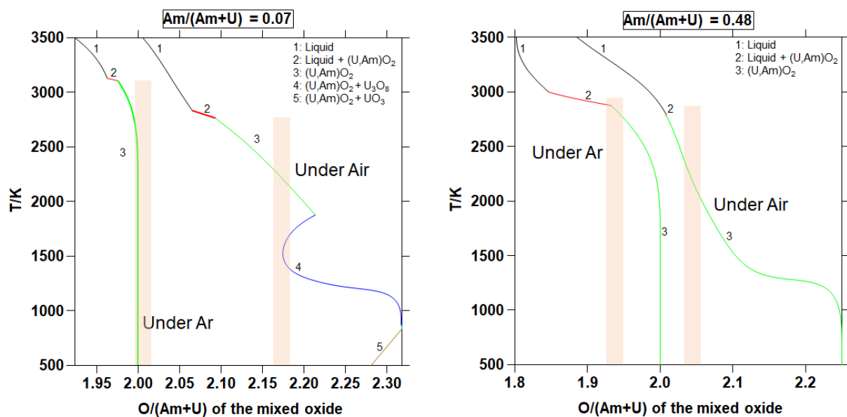
Figure 12. Cooling paths in a temperature-O/M ratio graph. The stable phases in each domain are specified on the figure. The orange rectangular areas are centred on the O/M ratio determined experimentally (at room temperature).
