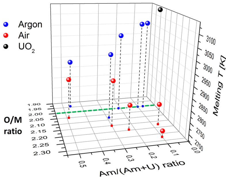
Figure 11. Melting temperature versus the final (room temperature) O/M-Am/M compositions.
