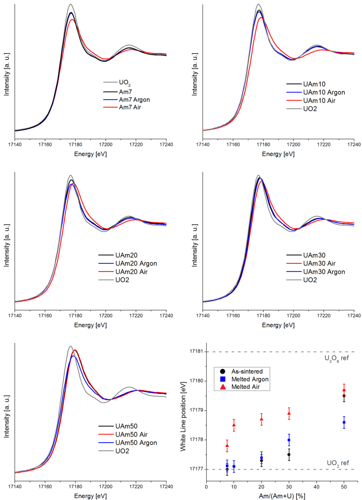
Figure 8. XANES spectra collected at the U-L 3 edge of Am on (U,Am)O 2 oxides, before and after melting. Bottom right: observed white lines.
