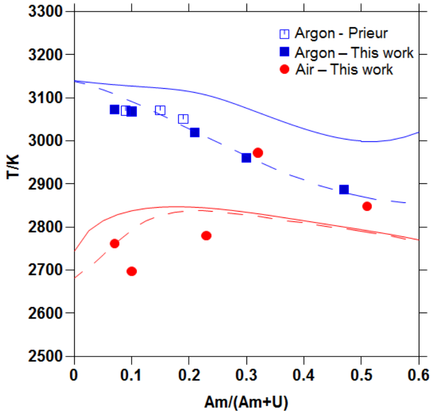
Figure 10. Computed solidus (- -) and liquidus (—) temperatures under argon (blue) and air (red), compared to the experimental points of Prieur [6] and this work.
