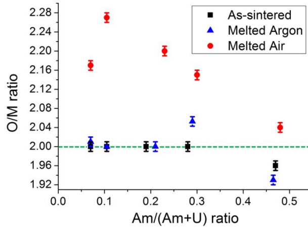
Figure 9. Composition of the melted samples obtained by XAS investigation.
