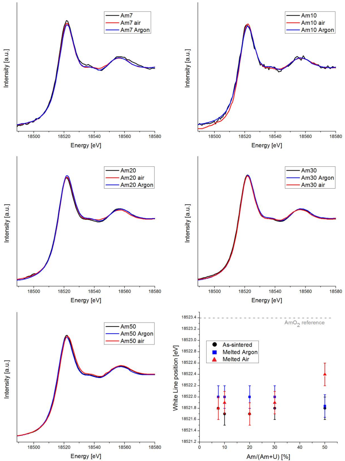
Figure 7. XANES spectra collected at the Am-L 3 edge of Am on (U,Am) 2 O x oxides, before and after melting. Bottom right: observed white lines.
