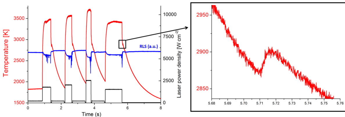
Figure 1. Thermogram (red), laser power profile (black) and reflected light signal (blue) recorded in a laser melting measurement in argon on the Am50 sample.
