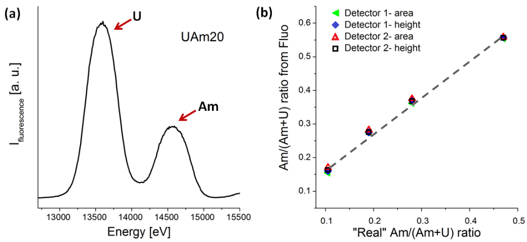
Figure 5. (a) Fluorescence X-ray spectrum of the Am20 sample for incident X-ray with E = 18.9 keV. (b) Am/(Am+U) ratio obtained by fluorescence spectroscopy for the as-sintered samples.
