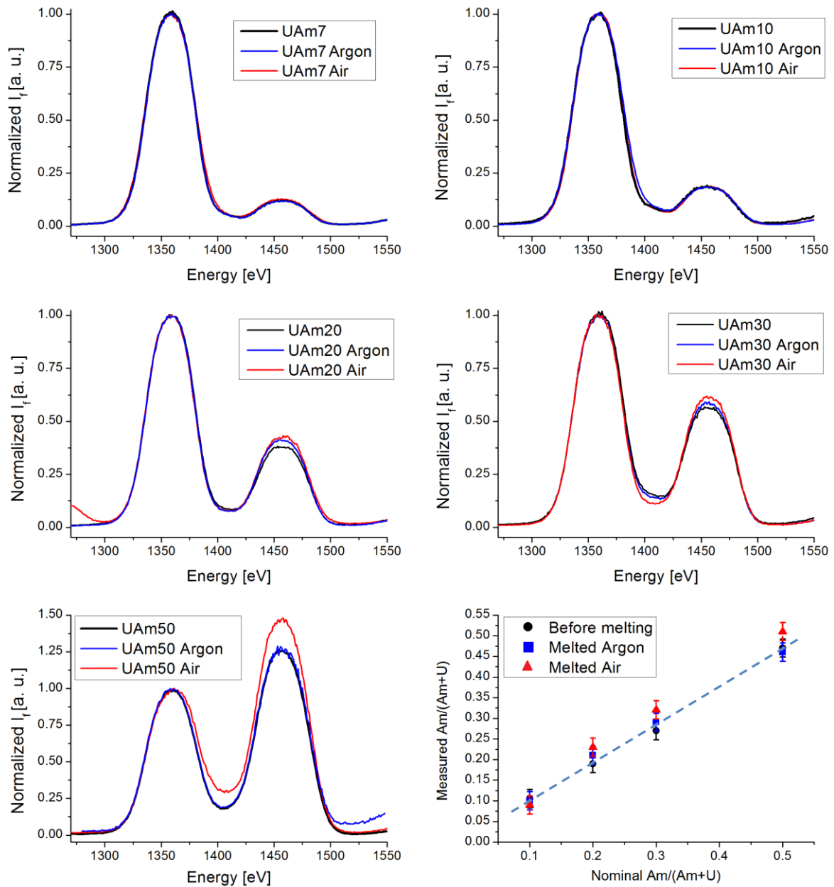
Figure 6. Comparison of the fluorescence spectra obtained on the as-sintered and melted samples of each composition and (bottom-right) resulting Am/M ratio vs the nominal Am/M.
