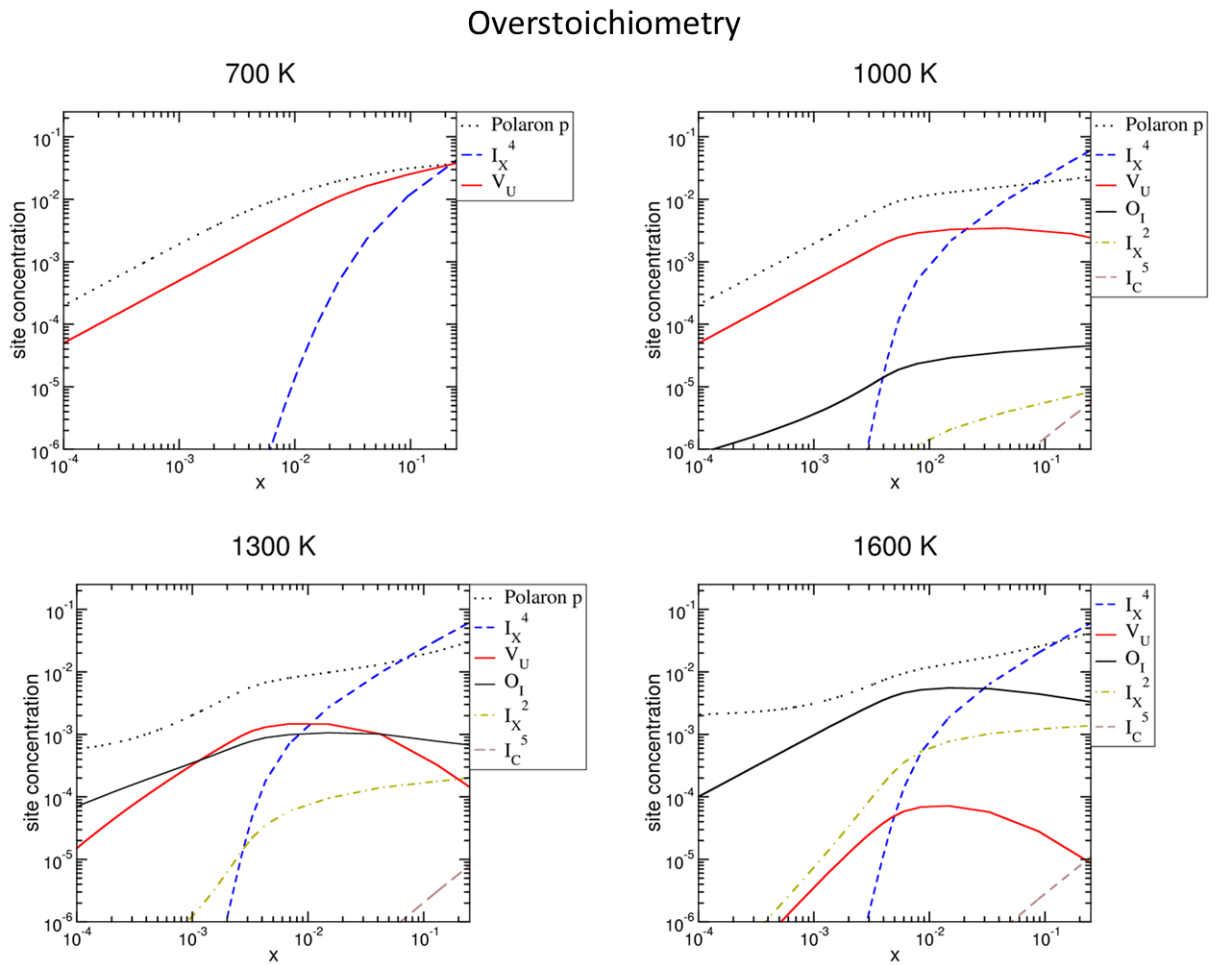
Figure 3: Concentrations of defects as a function of x in \text{UO}_{2+x} for different temperatures. Note that uranium vacancies (resp. oxygen interstitials) are dominant at low (resp. high) temperatures. For clarity, we only report the total concentration for each defect where all the possible charge states have been summed up.
