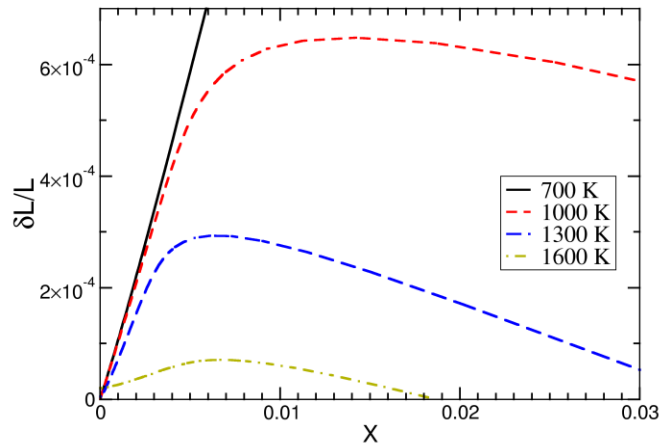
Figure 5: Elongation of UO_{2+x} relative to stoichiometric UO_2 as a function of x for different temperatures.
