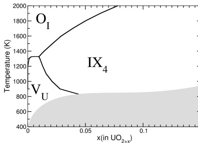
Figure 4: Dominant defect as a function of temperature and deviation from stoichiometry ( x ) in UO_{2+x} ; The shaded area indicates the miscibility gap[48] between UO_2 and U_4O_9 (inaccessible compositions).
