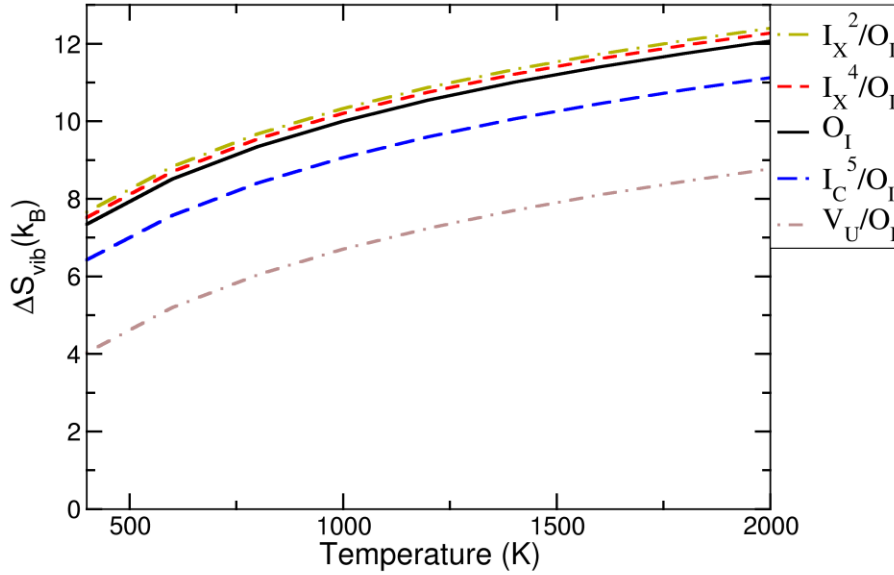
Figure 2 : Formation entropy of hyperstoichiometric defects from SMTB-Q calculations. The entropy \Delta S_{f-vib}^{m,n} are divided by the number of oxygen interstitials they contain or amount to.
