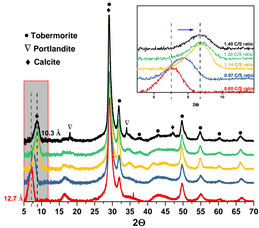
Figure 2. Powder XRD patterns of the different C-S-H samples (From bottom to top: 0.80, 0.97, 1.14, 1.30 and 1.40 CSH RH=60%).
