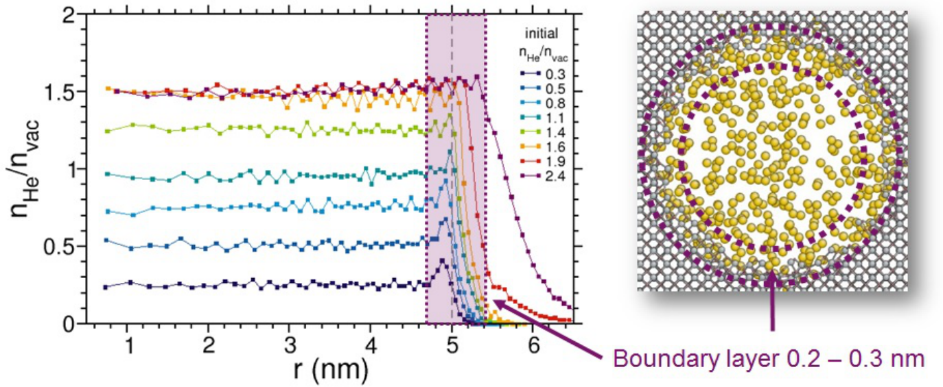
Figure 4: The left figure is the concentration profiles in a 10 nm diameter bubble calculated at 500 K as a function of the distance from the bubble center for different initial He concentration. The grey vertical dashed line represents the initial surface of the bubble. The figure on the right represents a snapshot of the atom spatial distribution for an initial concentration of 1.4 n_{\text{He}}/n_{\text{vac}} .
