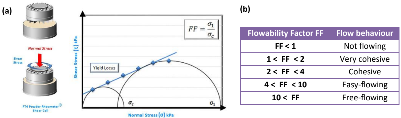
Figure 3 : Principe shear test and yield locus (a); classification of flowability factor FF (b) [16] .
