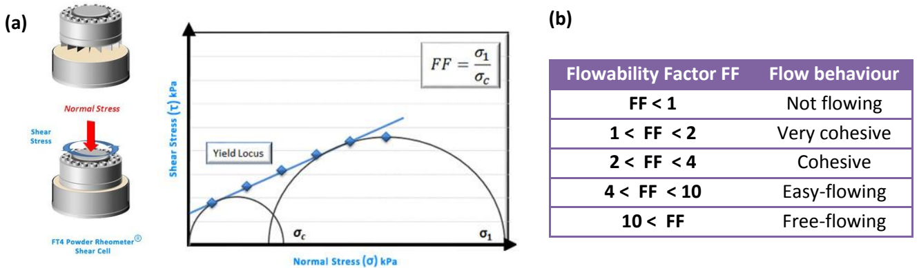
Figure 3 : Principe shear test and yield locus (a); classification of flowability factor FF (b) [16] .
