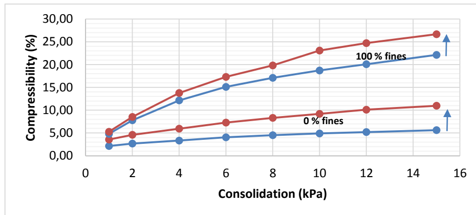
Figure 12 : Compressibility test before and after the VFR test (For 0% and 100% of fines).
