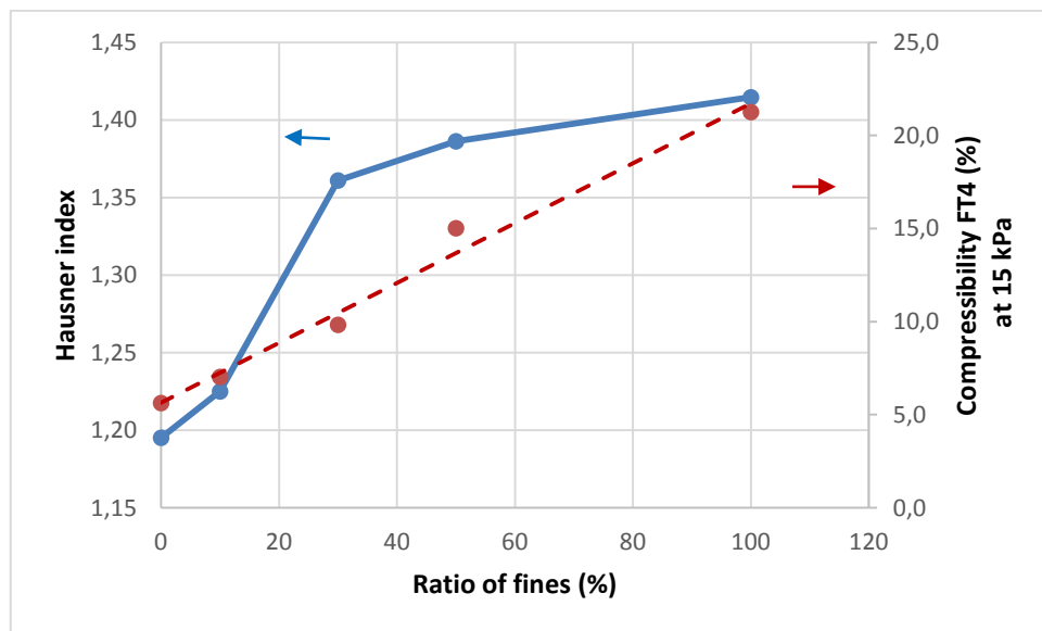
Figure 5 : Hausner index (blue) and compressibility (red) FT4 versus quantity of fines.
