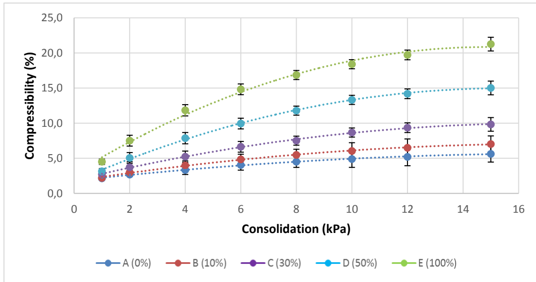
Figure 4 : Compressibility as function of consolidation.
