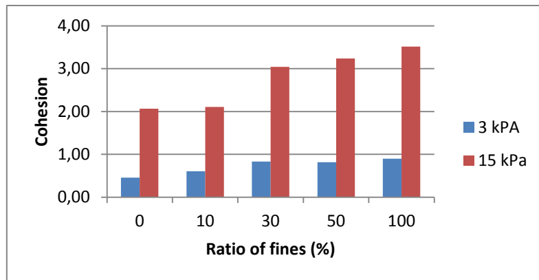
Figure 8 : Evolution of cohesion as function of quantity of fines (for pre-consolidation stresses 3 kPa and 15 kPa).
