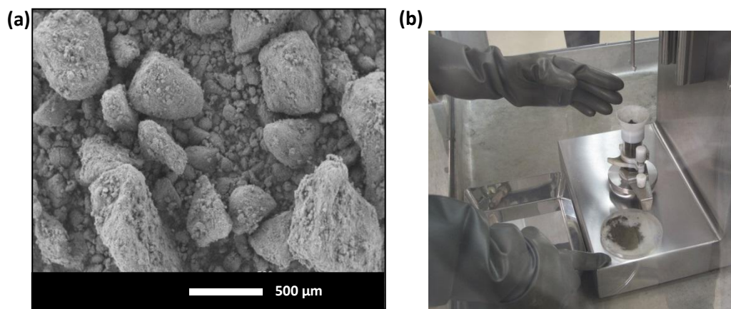
Figure 1 : SEM image (SE Mode), uranium dioxide powder (a) and powder handling in a glove box (b).
