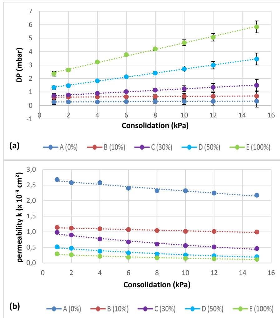
Figure 9 : Evolution of DP (a) and permeability k (b) as function of consolidation for different quantities of fines.
