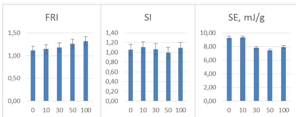
Figure 11 : VFR tests and the different indexes as function of quantity of fines (BFE, NBFE, FRI, SI and SE).
