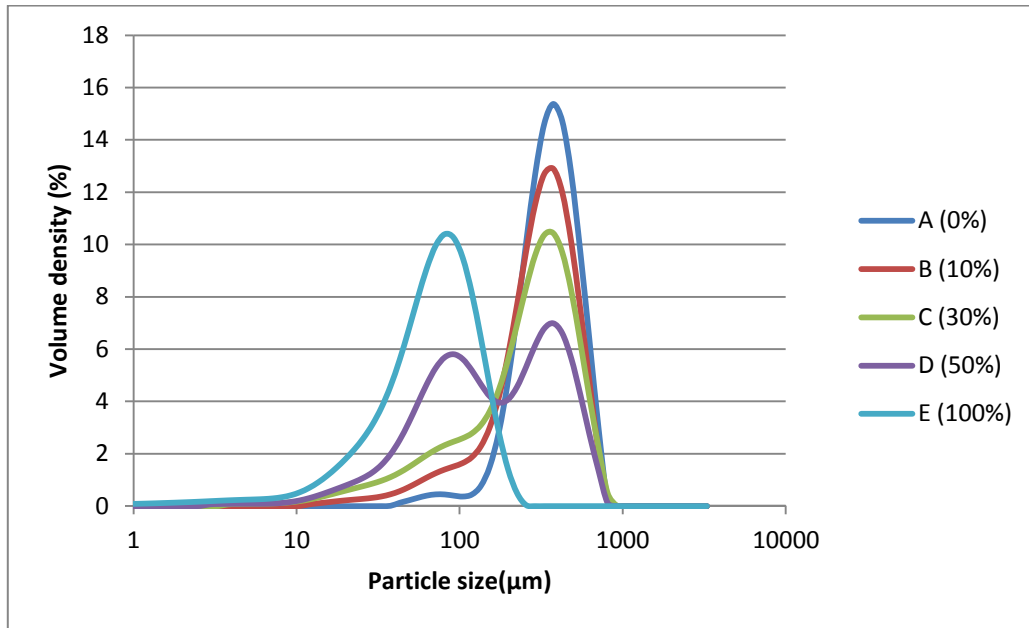
Figure 2 : Different particle size distributions (volume fraction).
