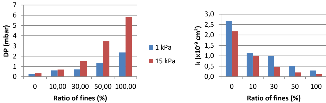
Figure 10 : Pressure drop DP (left) and permeability k (right) versus quantity of fines (for 1 kPa and 15 kPa).
