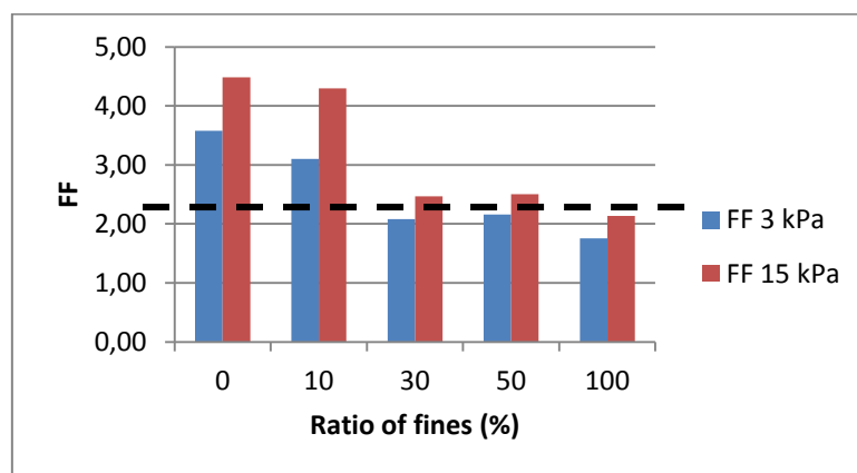
Figure 7 : Variation of the Flow factor FF as function of quantity of fines.
