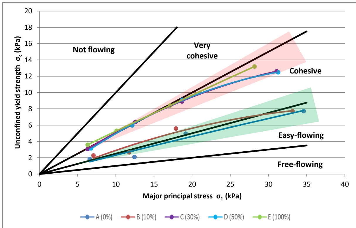
Figure 6 : Flow functions for the various particle size distributions.
