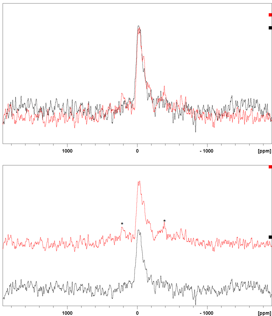
Figure 7 (a) Overlaid ^{25}\text{Mg} MAS NMR spectra of unleached MW25 (black) and MgEM (red) glasses obtained at 52.05 MHz with 54200 \pi/18 pulse and 0.1 s pulse delay and 102400 \pi/18 pulses and 1.5 s pulse delay, respectively. The spinning speed is the same at 14 kHz. Spectra are referenced to 1M \text{MgCl}_2 solution as 0 ppm; (b) The same spectra as shown in (a) stacked so that the spinning sidebands on MgEM spectrum can be seen (denoted by asterisks)
