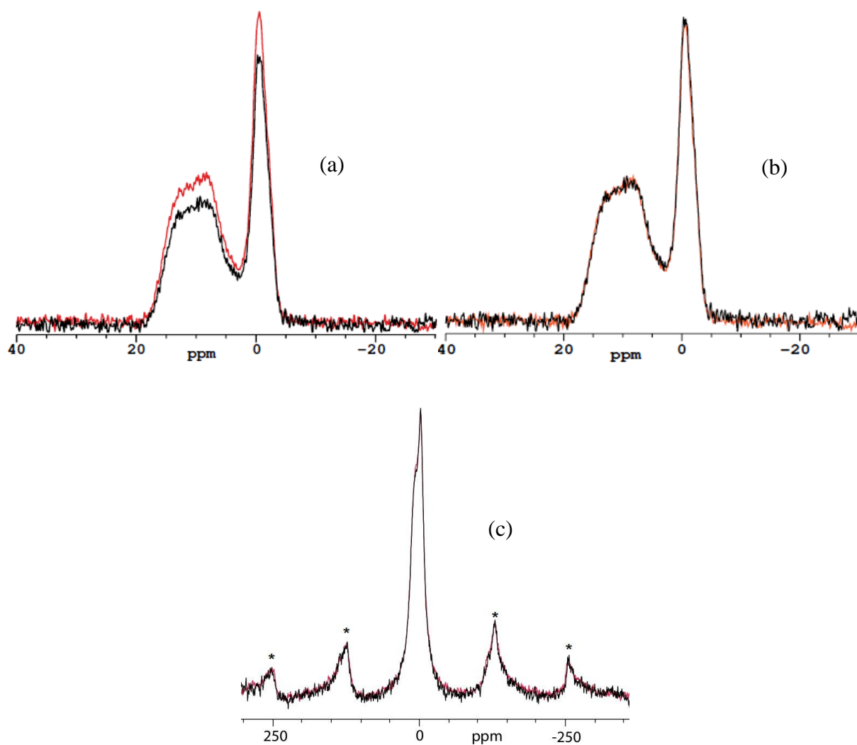
Figure 3 ^{11}\text{B} MAS NMR spectra of MgEM glass before (red) and after (black) a 112-day leaching experiments, (a) on an absolute scale and (b) normalised to make the ^{[4]}\text{B} peak intensities equal, obtained with the same experiment setup as in Figure 2; (c) ^{11}\text{B} MAS NMR spectra of MW25 glass before (red) and after (black) a 112-day leaching experiments normalised to make the ^{[4]}\text{B} intensities equal
