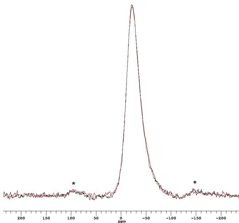
Figure 4 ^{23}\text{Na} MAS NMR spectra of simplified CaEM (red) and MgEM (black) glasses obtained at 105.82 MHz with 8192 \pi/18 pulse and 1.0 s pulse delay. Spinning speed was 12 kHz in both cases and the spinning sidebands are denoted by asterisks. Spectra are referenced to 1M \text{NaNO}_3 solution
