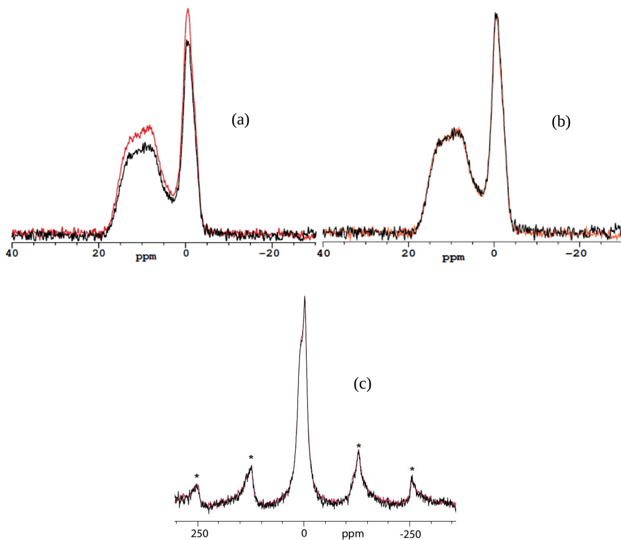
Figure 3 ^{11}\text{B} MAS NMR spectra of MgEM glass before (red) and after (black) a 112-day leaching experiments, (a) on an absolute scale and (b) normalised to make the ^{11}\text{B} peak intensities equal, obtained with the same experiment setup as in Figure 2; (c) ^{11}\text{B} MAS NMR spectra of MW25 glass before (red) and after (black) a 112-day leaching experiments normalised to make the ^{11}\text{B} intensities equal
