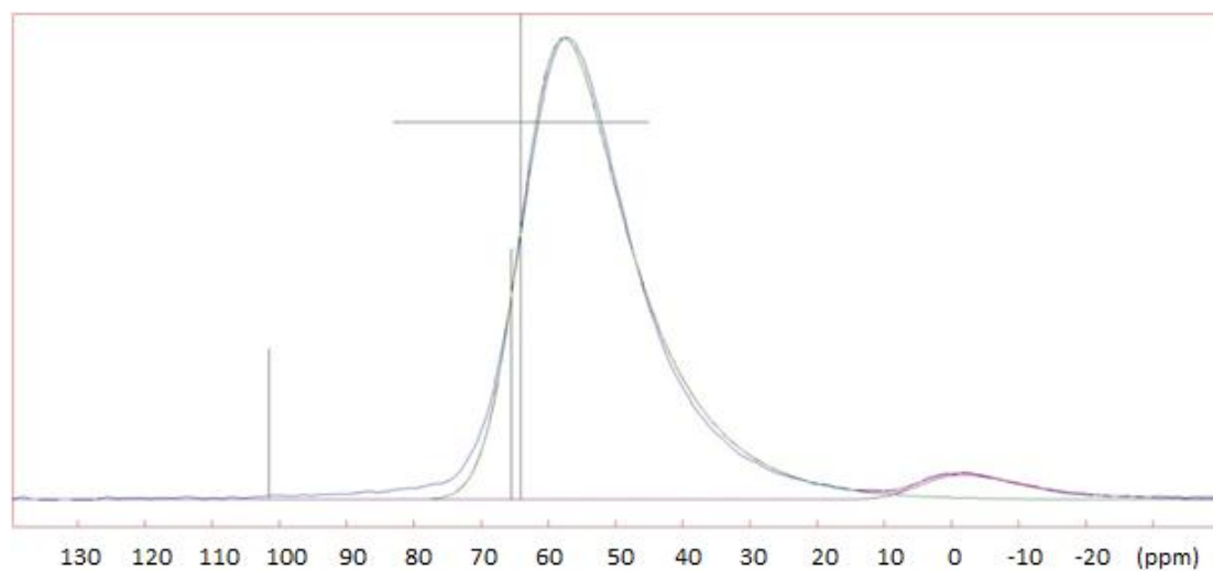
Figure 6 Curve fitting of the CaEM ^{27}\text{Al} MAS NMR spectrum with 2 CzSimple lines: ^{[4]}\text{Al} in green and ^{[6]}\text{Al} in purple.
