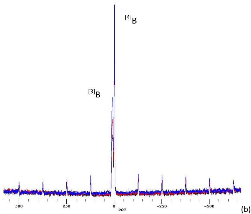
Figure 2 ^{11}\text{B} MAS NMR spectra of the simplified glasses CaEM (black), Mg50Ca50 (red) and MgEM (blue) obtained at 160.34 MHz. (a) The central transition lineshape of ^{[4]}\text{B} and ^{[3]}\text{B} peaks; (b) The full spectra that manifest the sidebands of ^{11}\text{B} satellite transitions. The intensities of the ^{[4]}\text{B} peaks are normalised for comparison of the relative proportion of trigonal ^{[3]}\text{B}
