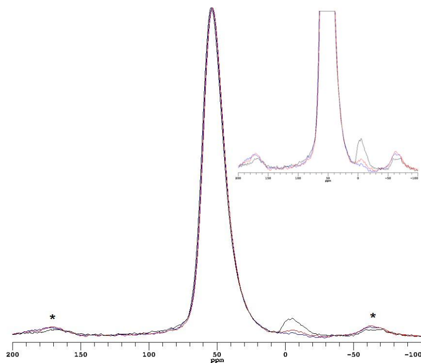
Figure 5 ^{27}\text{Al} MAS NMR spectra of simplified CaEM (black), Mg50Ca50 (blue) and MgEM (red) glasses obtained at 130.22 MHz with 8192 \pi/18 solid pulse and 0.3 s pulse delay. The four-coordinated Al peaks are normalised for comparison of the relative proportion of six-coordinated Al. Spinning speed is 15 kHz in all cases and the spinning sidebands are denoted by asterisks. Spectra are referenced to 1M \text{Al}(\text{NO}_3)_3 solution
