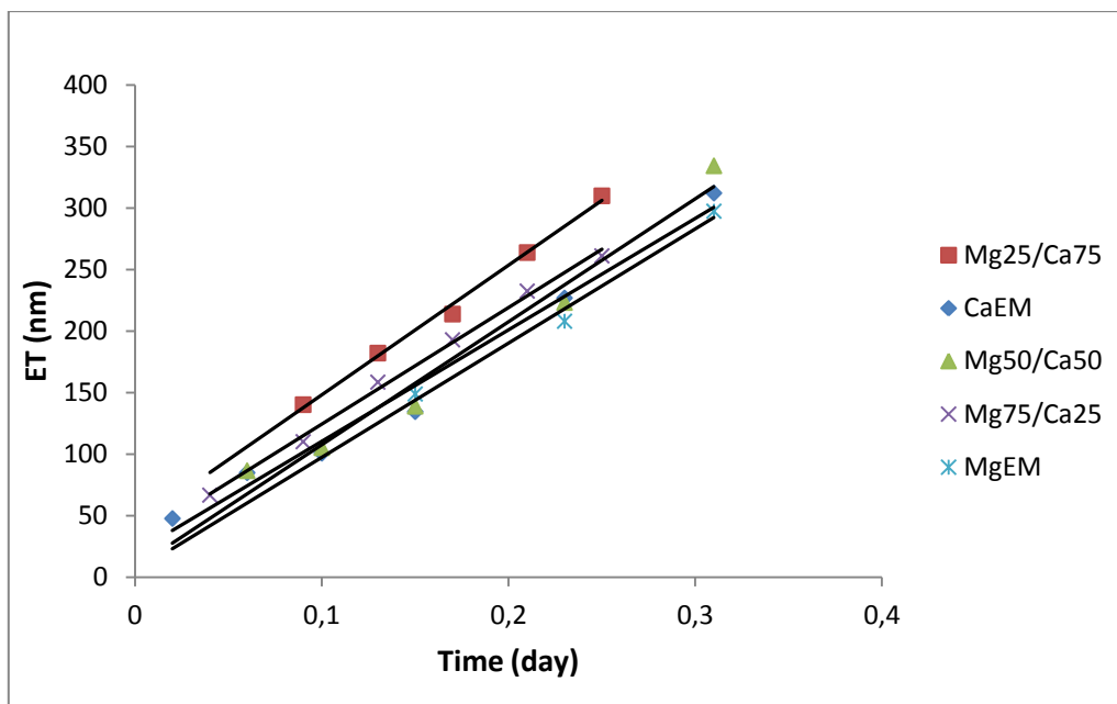
Figure 8 Effective dissolved thickness (ET) of simplified glasses as a function of time in the initial dissolution rate experiments based on Si concentration in the leachate
