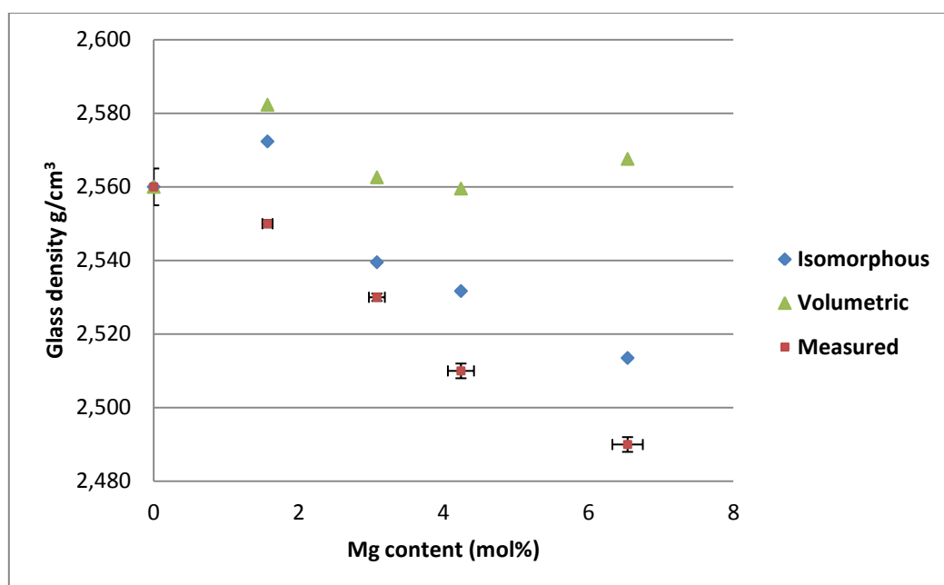
Figure 1 The measured glass densities as a function of Mg content and predicted densities based on: (i) an isomorphous substitution of Ca for Mg according to the molar mass of CaO and MgO; and (ii) a volumetric substitution which also takes the molar volumes of CaO and MgO into account; see Section 4.1 for details
