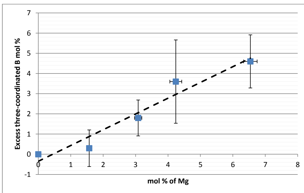
Figure 9 The linear fit (dashed line) of the amount of boron that transform from four-fold coordination to three-fold coordination on substitution of Mg for Ca per 100 moles of cations (filled square)
