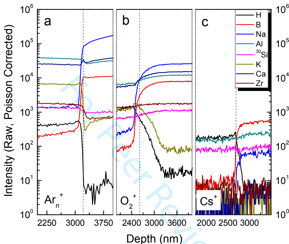
Figure 2. Depth profiles of several ion species of interest on corroded ISG glass in positive (with \text{Ar}_n^+ , \text{O}_2^+ sputtering) and negative (with \text{Cs}^+ sputtering) ion modes: sputtering beams were 20 keV \text{Ar}_n^+ (a), 2 keV \text{O}_2^+ (b) and 2 keV \text{Cs}^+ (c) with the current ratio of 100%; analysis beam was 25 keV \text{Bi}^+ . The dashed lines refer to the alteration layer-pristine glass interface. Common settings with reasonable sputtering rate and depth resolution in ToF-SIMS analysis were used. The ion intensities were all Poisson-corrected for dead-time correction during the analysis. The measured depths of the alteration front varied from 2700 nm to 3200 nm in different analysis areas, possibly due to an inhomogeneous thickness of the altered layers as depth profiling analysis using the above sputtering beams were conducted at different locations of the same sample.
