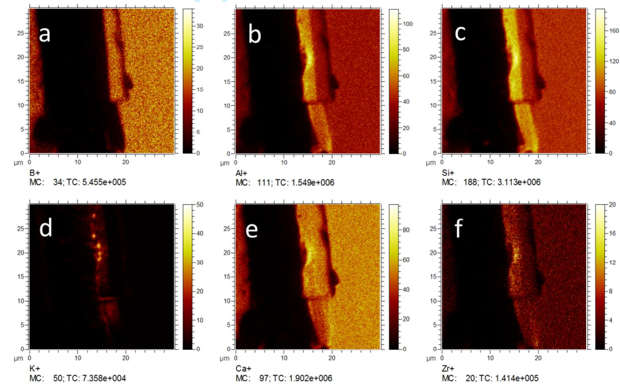
Figure 6. ToF-SIMS images of (a) B^+ , (b) Al^+ , (c) Si^+ , (d) K^+ , (e) Ca^+ and (f) Zr^+ ions. These images were collected simultaneously with those in Figures 5c and 5d using a 1 keV O_2^+ auxiliary sputtering beam at a current density of 0.89\text{ A/m}^2 .
