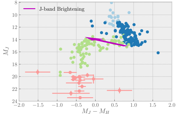
Figure 10. Color magnitude diagram M_J as a function of (M_J - M_H) . The magenta arrow indicates the J-band brightening in the color magnitude diagram. The photometry is extracted from Faherty et al. (2012); Dupuy & Liu (2012); Dupuy & Kraus (2013); Beichman et al. (2014). The different colors from top to bottom correspond to respectively, M, L, T, and Y dwarfs.
