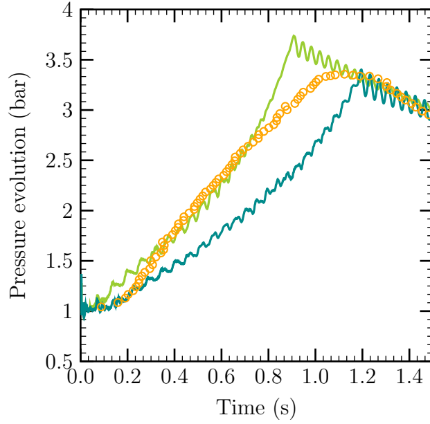
Figure 16: Test 7 (no spray). Pressure evolution for hydrogen-air mixture ( x_{H_2} = 0.16 ), with p_{ini} = 1.013 bar, H_1 = 1700 W/m 3 /K, H_2 = 425 W/m 3 /K, K_0 = 5.73 m/s. The experimental results are given in (○). Comparison between the coarse mesh \Delta x = 10 cm (—) and the finer mesh \Delta x = 5 cm (—)
