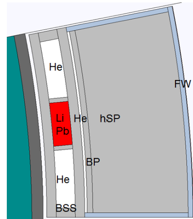
Fig. 3. Radial – toroidal cut of the inboard segment; BZ is closed by the FW, caps and BP, the internal He manifold behind the BP supply He in hSP (He comes from the FW output); BSS contains two helium manifolds which supply the FW and one LiPb manifold which directly supply the BZ
