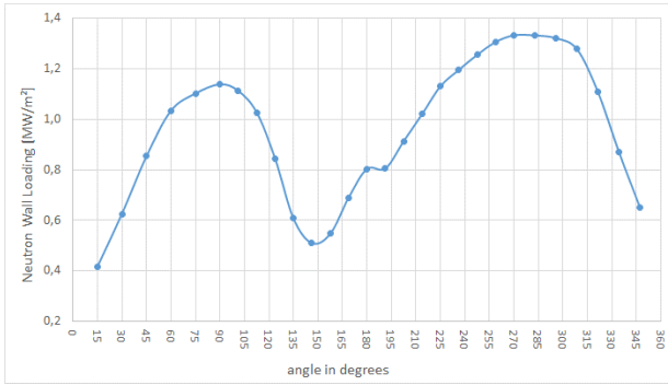
Fig. 4 NWL poloidal profile
