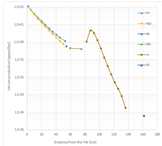
Fig. 8 helium production radial profile at inboard
