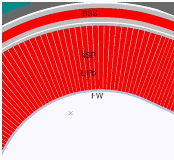
Fig. 2 Radial – poloidal cut of the upper part of inboard segment (color legend: LiPb – red, eurofer – gray, VV 1 st layer – deepgray, VV 2 nd layer – darkcyan). (For interpretation of the references to colour in this figure legend, the reader is referred to the web version of this article.)
