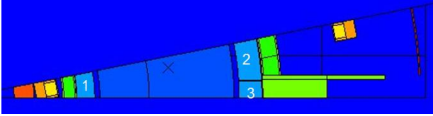
Fig. 1. Radial – toroidal cut of the DEMO 2017 half sector ( 11.25^\circ ); #1 inboard BB segment, #2 outboard BB lateral segment, #3 outboard central segment
