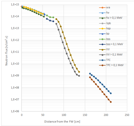
Fig. 5 neutron flux radial profile at inboard
