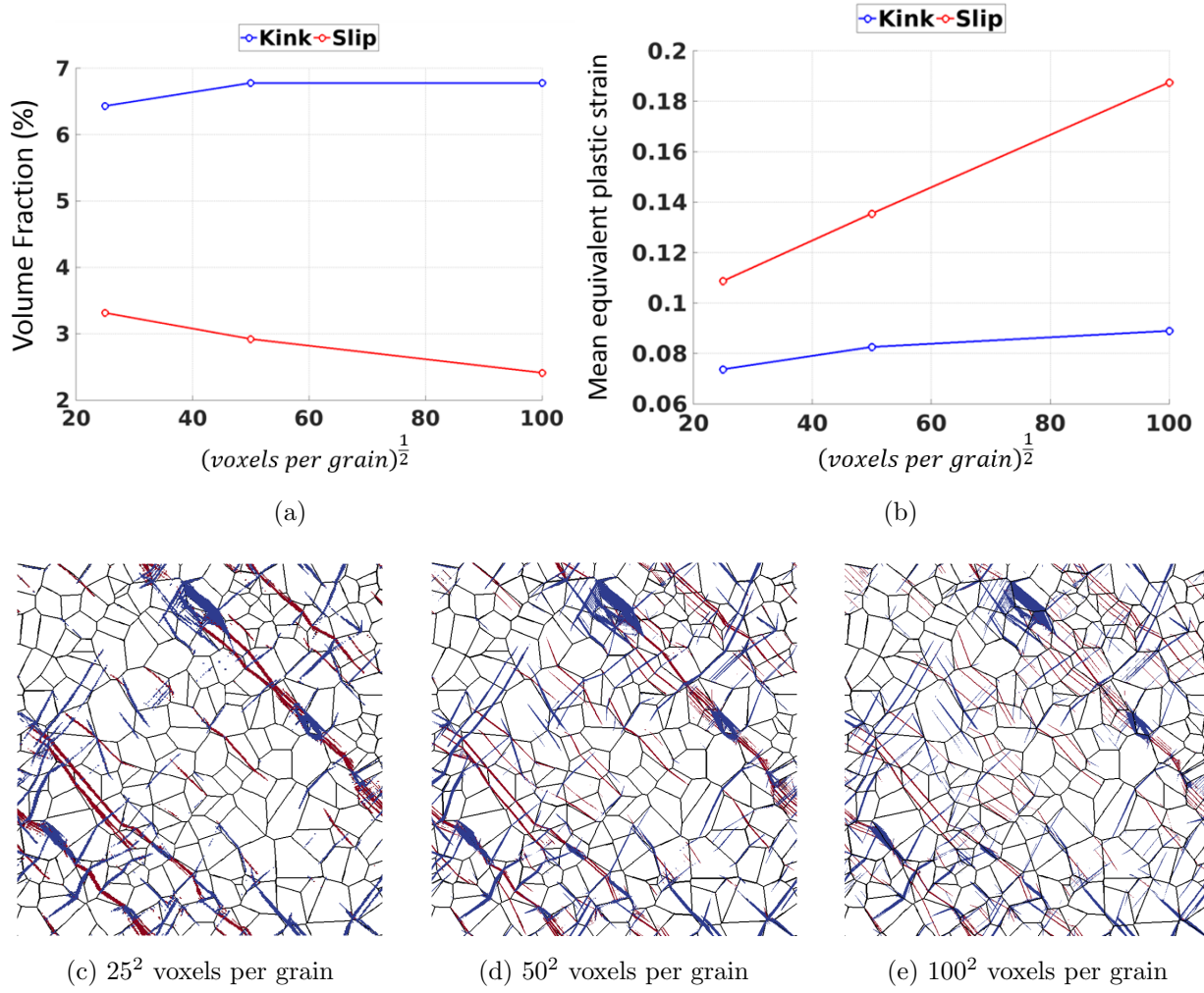
Figure 6: Influence of grid resolution on slip (red) and kink (blue) bands volume fraction (a) and mean equivalent plastic strain (b) for the 3 in-plane slip systems 2D polycrystal after 1% overall strain. (c - e): associated localization maps.
