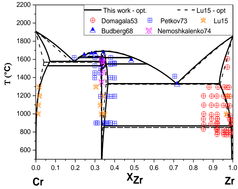
Figure 3: Calculated Cr–Zr system compared to experimental data.
